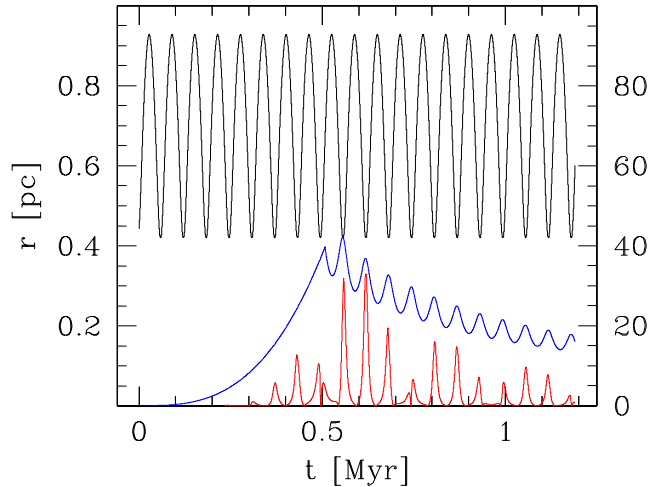
Figure 3. Orbit of a sample star in simulation R14.4lm6rh1 (left-hand panel). The location of the gas is marked by the red area. The corresponding evolution of the distance from the cluster centre (black), the proto-stellar disc truncation radius (blue), and the accretion rate (red) are shown in the right-hand panel.
