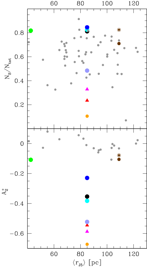
Figure 6. Fraction of SP (top panel) and A_2^+ parameter (bottom panel) measured in the last snapshot of all the simulations run within the cooling flow scenario. Grey points represent the observational fractions for the Galactic GCs (from Milone et al. 2017; Dalessandro et al. 2019). The colour code is described in the last column of Table 1. Circles and triangles represent simulations with and without primordial mass segregation. The symbol size is proportional to the initial Roche lobe filling factor r_h/r_J .
