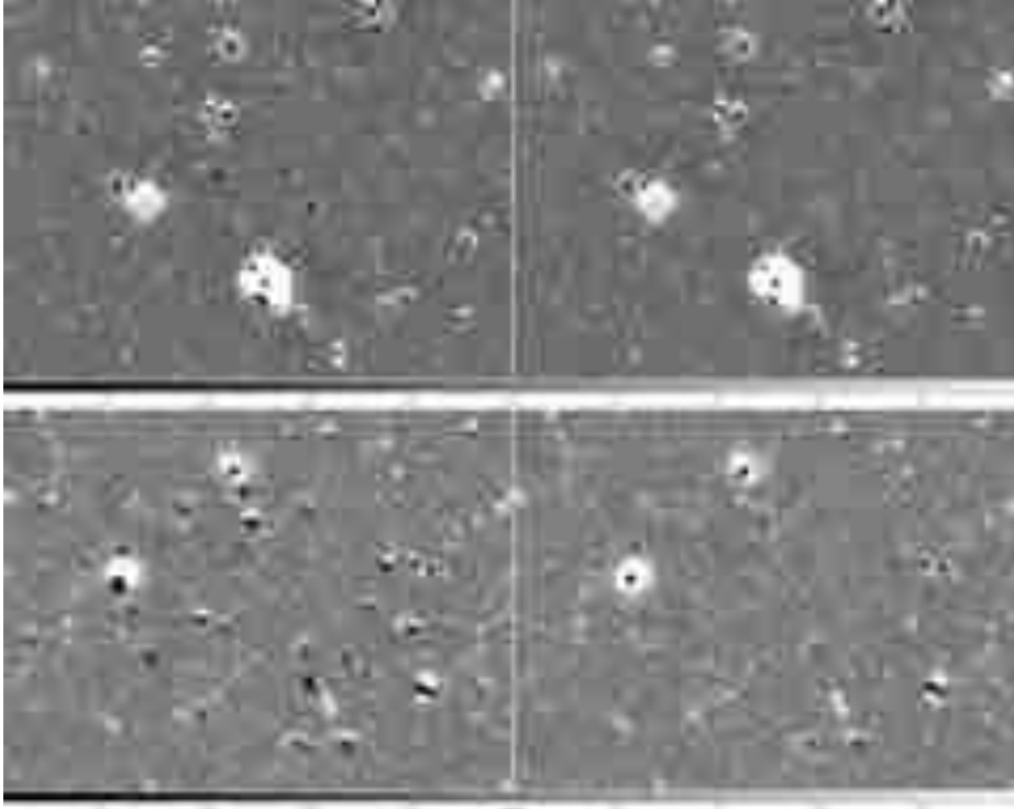
Fig. 18. UDS I -band TFIT versus T-PHOT comparison. The panels on the left show two small patches of the official CANDELS residual image obtained using T-FIT. The residual images of the same regions are showed in the right panels , this time obtained using T-PHOT with cells-on-objects method and improved local kernel registration. We note the disappearance of many spurious black spots.
