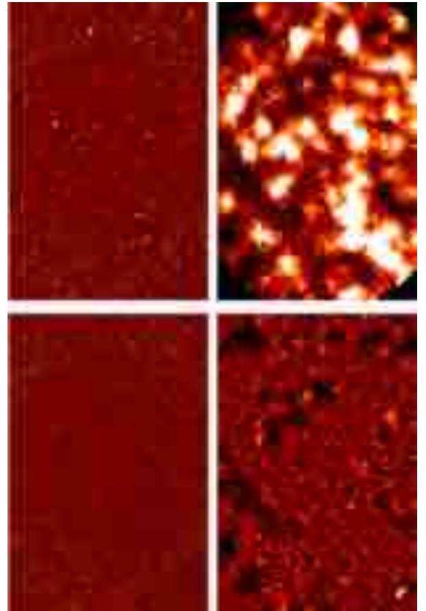
Fig. 19. Results from a test run using T-PHOT with unresolved priors on FIR/sub-mm real dataset. Upper row, left to right: SCUBA-2 450\ \mu\text{m} ( FWHM = 7.5'' ) and Herschel 500\ \mu\text{m} ( FWHM = 36'' ) images of the COSMOS-CANDELS fields. Lower row, left to right: residuals for the two fields, obtained with T-PHOT runs using a list of 24 + 850\ \mu\text{m} priors. See text for details.
