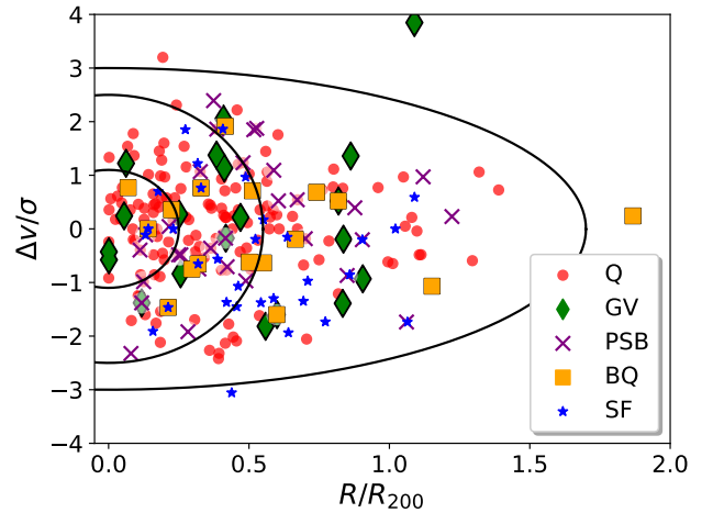
Figure 11. The distribution of galaxies with M > 10^{10.2} M_{\odot} and spectroscopic redshifts in phase space, as defined by Muzzin et al. (2014) . The solid contours represent the same phase space bins adopted by Muzzin et al. (2014) .
