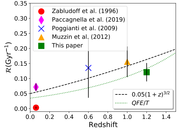
Figure 15. The rate of cluster-driven quenching, is calculated from Equation 5 for the BQ population with M \gtrsim 10^{10} M_{\odot} at three redshifts, from the sources indicated in the legend. We assume that \tau_{PSB} = 0.5 \text{ Gyr} is constant. The dashed line shows an arbitrarily normalized timescale that evolves inversely with the dynamical time. The dotted line represents the rate evolution implied by a constant QFE=0.4 (Appendix A), assuming the cluster forms at z = 3 .
