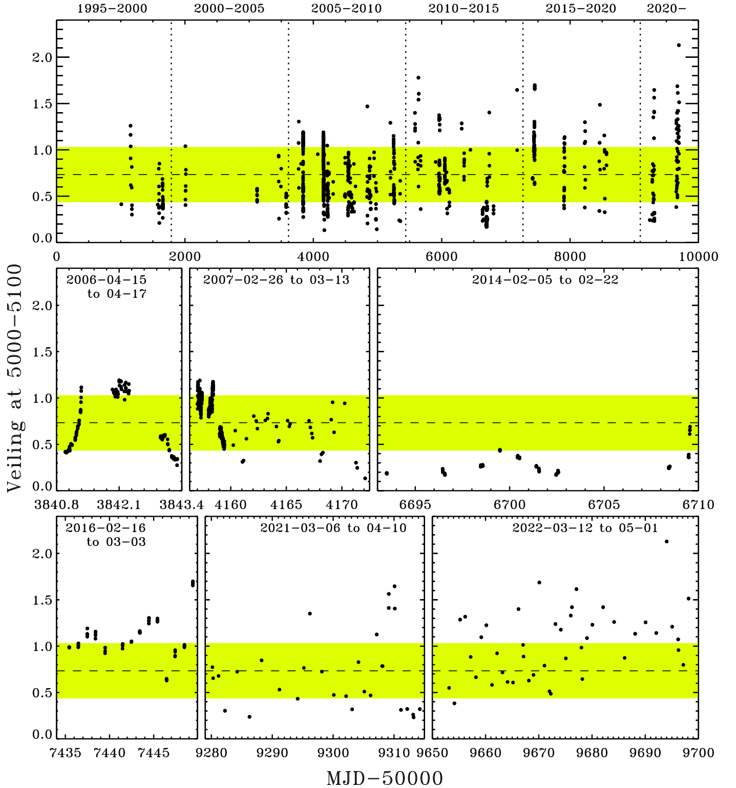
Figure 15. The full veiling lightcurve (top), with specific segments highlighted in the bottom six panels, with average veiling (horizontal line) and standard deviation (shaded yellow region). In the six panels, the date range in the x -axis differs in each plot.
