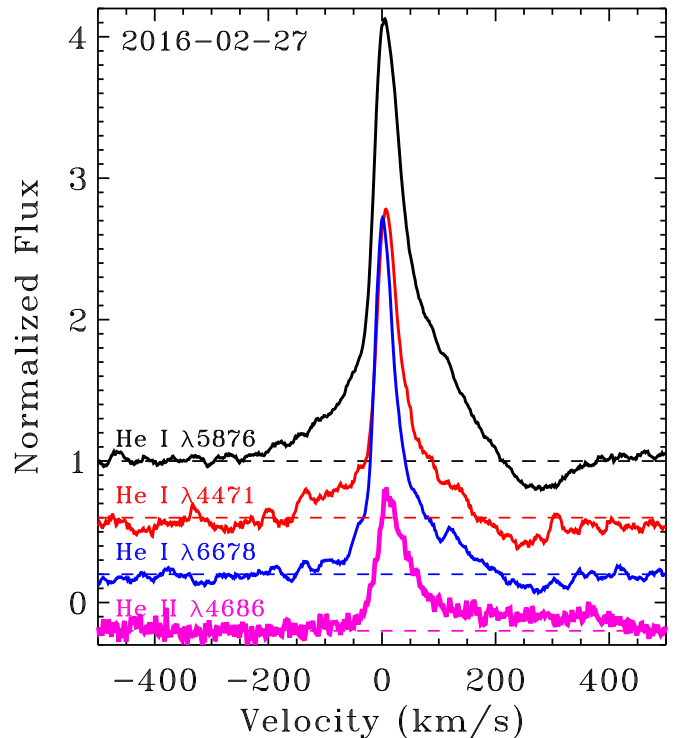
Figure 13. He I absorption, seen here to \sim 300\text{--}400 \text{ km s}^{-1} in three lines on 2016 February 27, an epoch with strong accretion. The He II \lambda 4686 line (bottom, pink) has emission that extends out to 450 \text{ km s}^{-1} .
