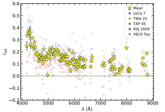
Figure 5. The zero-point of relative veiling as a function of wavelength. Yellow stars represent the final r_{\text{zpt}} determined by averaging the individually measured r_{\text{zpt}} from different stellar templates in colored dots in the background. The shape resembles the relation between relative veiling and wavelength.
