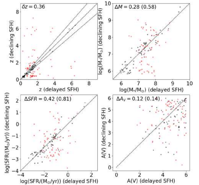
Fig. B.3. Same as Figure A.2, but comparing two different SFHs, i.e. delayed and declining.
