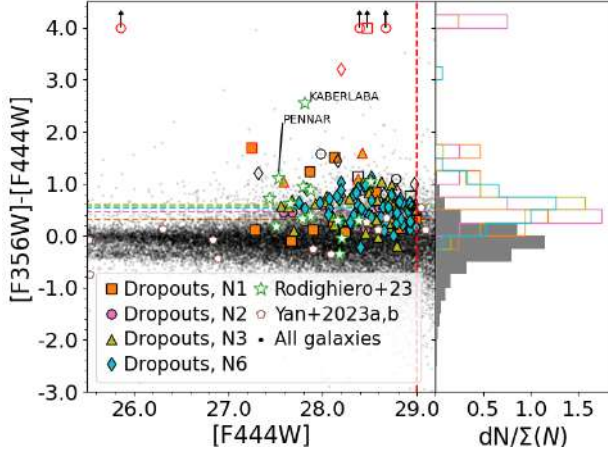
Fig. 4. Left: [F444W] magnitude vs. [F356W] - [F444W] colour of the F200W -dropout sample in the four NIRC2 pointings (coloured points and histograms, named N1, N2, N3, and N6) and for full CEERS sample (black dots and grey histogram). Points with a red edge are objects in the F200W -dropout-extra sub-sample. Empty symbols indicates objects in our sample with a S/N < 3 in the F356W filter and we assigned, for visual purposes, a colour of [F356W] - [F444W] = 4 to galaxies with redder colours. We also report the sample of F200W -dropouts by Rodighiero et al. (2023, green empty stars), highlighting their two candidates at z > 10 , namely KABERLABA and PENNAR, and the sample by Yan et al. (2023a, brown empty pentagons). Right: normalised [F356W] - [F444W] colour density distribution. Each histogram is normalised so that its integral is equal to one.
