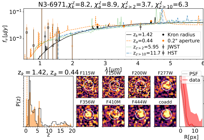
Fig. 3. Example of the SED fitting applied to a galaxy (N3-6971) in our F200W -dropout sample. In the top panel we report the photometry and the best fit derived with the 0.2'' -radius aperture (orange) and the Kron aperture leaving the redshift free (black), forcing it at z > 2 (green dotted) and at z > 10 (blue dash-dotted). Empty symbols indicate fluxes with S/N < 3 . Similarly, in the bottom left panel we report the redshift probability distribution function (PDF) derived with the two photometric sets, with the peak values highlighted by vertical lines. On the bottom, we include eighth cutout images in the JWST filters and in the co-added F277W , F356W , and F444W band images. A white circle indicates the 0.2'' -radius aperture. On the bottom right we report the light profile of the target (red solid line and shaded area) compared with the observed PSF of the F444W filter (black dotted line).
