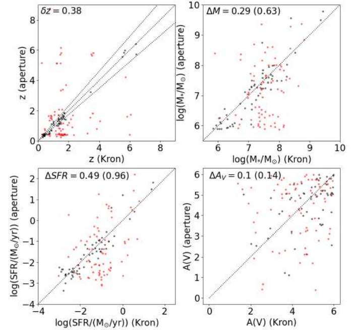
Fig. A.2. Comparison between the physical parameters derived using BAGPIPES based on photometry derived using a Kron aperture and a 0.2'' -radius aperture. From top left to bottom left: redshift, stellar mass, SFR and A(V) . Black dots show galaxies for which the redshift is well recovered, while red dots show redshift outliers, i.e. \delta z = |z_{\text{Kron}} - z_{0.2''}|/(1 + z_{\text{Kron}}) > 0.15 . On the top left of each panel we show the absolute difference between the physical properties derived with Kron and 0.2'' aperture, for galaxies with a good redshift and, in brackets, for the entire sample.
