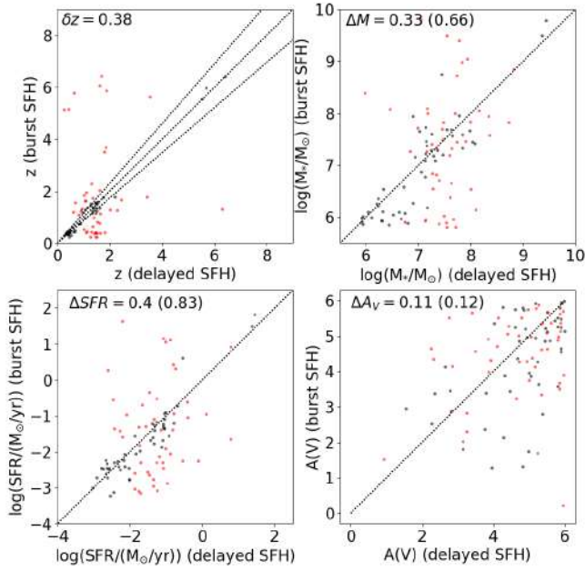
Fig. B.4. Same as Figure A.2, but comparing two different SFHs, i.e. delayed and a burst.
