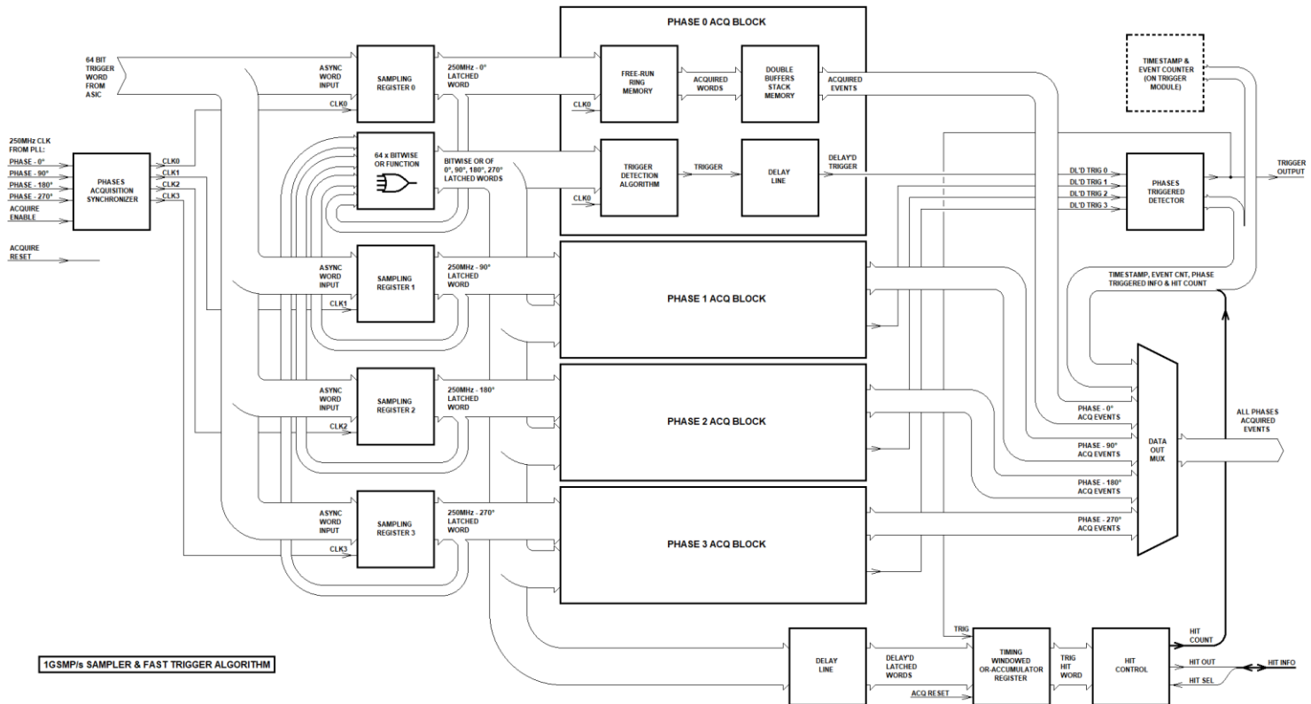
Fig 3: IP-Module with 1 GSMP/s sampling acquisition and fast trigger algorithm
