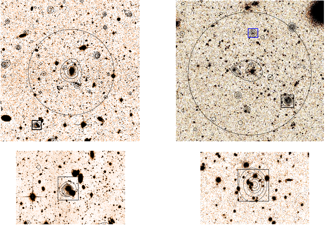
Fig. 7. Optical images (i band) of two XXL clusters overplotted with X-ray contours (0.5–2.0 keV). Left panels: XLSSC 041 (in XXL-N), a C1 cluster at z = 0.142 with an estimated mass of M_{500,MT} \sim 8.3 \times 10^{13} M_{\odot} and r_{500,MT} = 636 kpc. Right panels: XLSSC 561 (in XXL-S) a C2 cluster at z = 0.455 with an estimated mass of M_{500,MT} \sim 9.3 \times 10^{13} M_{\odot} and r_{500,MT} = 993 kpc. The boxes indicate the position of AGNs with spectroscopic redshifts concordant with the respective cluster redshift. The bottom panels are zoomed-in images of the AGNs found in the black boxes. Both these AGNs are found in overdense regions, where galaxy interactions and merging is probable.
