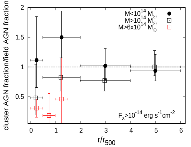
Fig. 5. Fraction of XXL bright cluster galaxies hosting an X-ray AGN for a flux-limited sample ( F_{X[0.5-10\text{ keV}]} > 10^{-14} \text{ erg sec}^{-1} \text{ cm}^{-2} ), divided by the field fraction. The results are plotted as a function of distance from the cluster centre. No AGN suppression is present in our low-mass cluster sample, in contrast to the results of Ehlert et al. (2014) on massive clusters. Error bars indicate the 1\sigma confidence limits for small numbers of events (Gehrels 1986).
