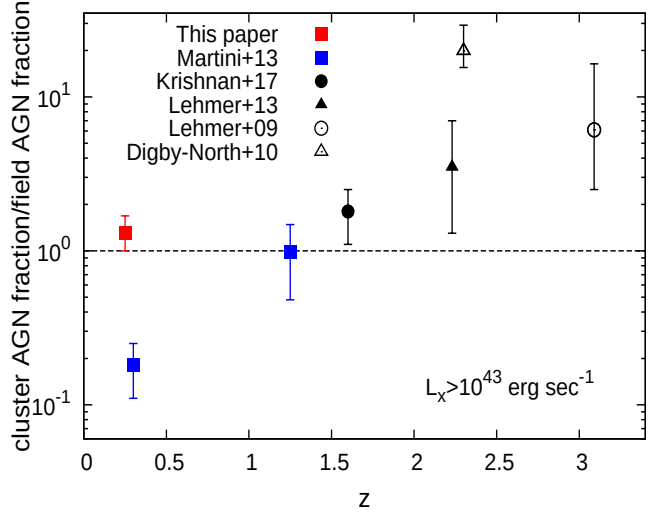
Fig. 9. Fraction of XXL bright cluster galaxies hosting an X-ray AGN ( L_{X[0.5-10\text{ keV}]} > 10^{43} \text{ erg sec}^{-1} ) within a 2r_{500} radius, divided by the field fraction. The results are plotted as a function of redshift. We overplot the results of similar analyses of cluster samples (blue) or individual high-redshift proto-clusters (black), as described in Sec. 5. Open symbols mark different luminosity limits used for the X-ray AGNs.
