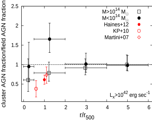
Fig. 4. Fraction of XXL bright cluster galaxies hosting an X-ray AGN ( L_{X[0.5-10\text{ keV}]} > 10^{42} \text{ erg sec}^{-1} ), divided by the field fraction. The results are plotted as a function of distance from the cluster centre. The sample is divided in two based on cluster mass. Error bars indicate the 1\sigma confidence limits for small numbers of events (Gehrels 1986). For comparison we plot results from the analyses of massive clusters by Martini et al. (2007, 8 clusters, 0.06 < z < 0.31 ), Koulouridis & Plionis (2010, 16 clusters, 0.07 < z < 0.28 ), and Haines et al. (2012, 26 clusters, 0.15 < z < 0.30 ). A significant AGN excess is found between 0.5r_{500,MT} and 2r_{500,MT} , at the 95% confidence level.
