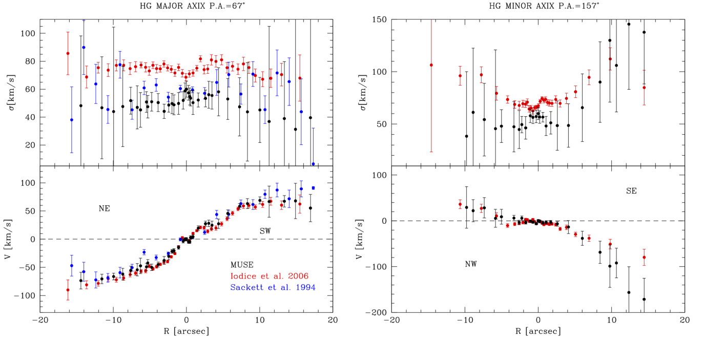
Fig. 6. Stellar kinematics along the major axis ( left panel ) and minor axis ( right panel ) of the HG in NGC 4650A derived by MUSE data (black points) in the Mgb wavelength region compared with the profiles obtained by Sackett et al. (1994), blue points, in the same region, and longslit spectra by Iodice et al. (2006), red points, in the CaT wavelength region.
