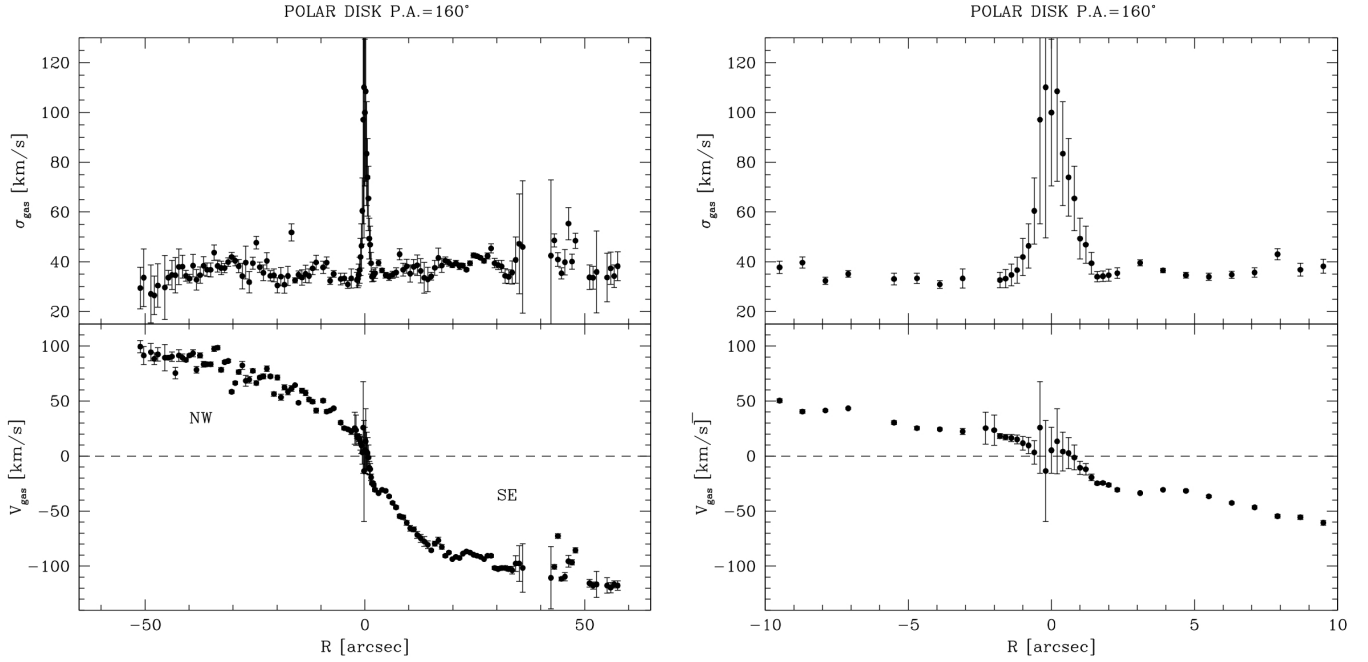
Fig. 8. Left panel: line-of-sight velocity (bottom panel) and velocity dispersion (upper panel) of the gas along the polar disk major axis, PA = 160°. Right panel: zoom of the gas rotation (bottom) and dispersion (upper) curves towards the centre of the galaxy.
