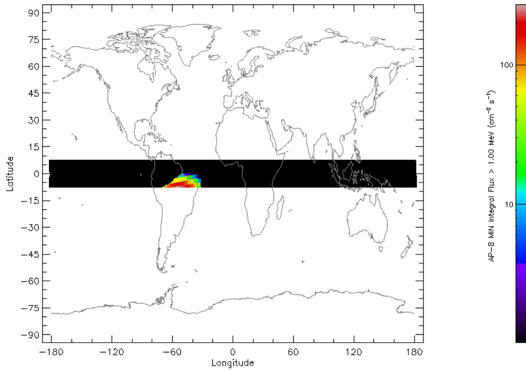
Figure 1: Map of the trapped proton flux at a XIFE orbit with 600 km altitude and 6° inclination. The flux is omnidirectional ( 4\pi sr) and is clearly concentrated in the SAA.
