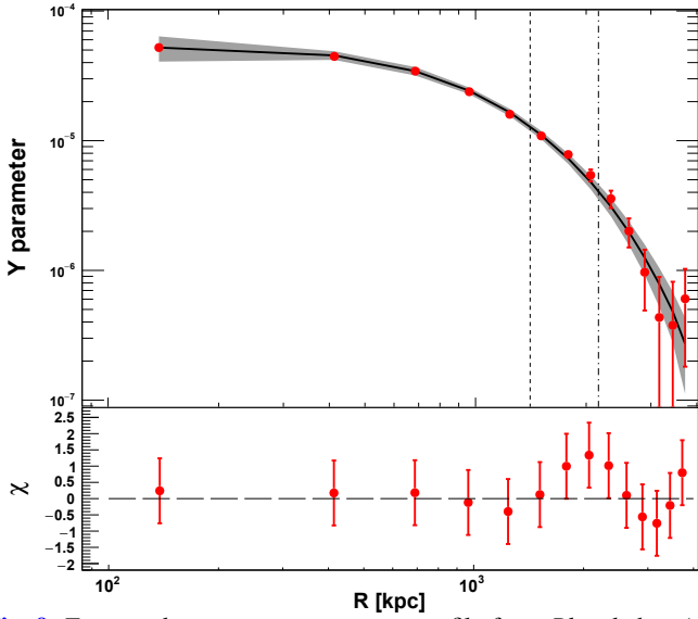
Fig. 9. Top panel: compton- y parameter profile from Planck data (red points). The gray solid line and shaded area show the best-fit profile convolved with the instrument PSF. The data points are correlated and the associated errors correspond to the square root of the diagonal elements of the covariance matrix. Bottom panel: residual of the fit to the Planck data. The dashed and dash-dotted vertical lines represent R_{500} and R_{200} , respectively.
