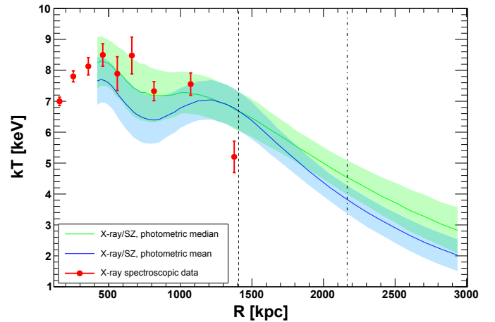
Fig. 11. Deprojected temperature profile. Red points: spectroscopic data (from Fig. 3) deprojected using the method of Ettori et al. (2010); green and blue: combined X-ray and SZ profile using the azimuthal median and azimuthal mean density profiles, respectively. The dashed and dash-dotted vertical lines represent R_{500} and R_{200} , respectively.
