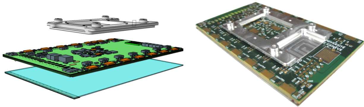
Figure 6. Views of the thermo-mechanical prototype of the FEE. From Ref. 5
