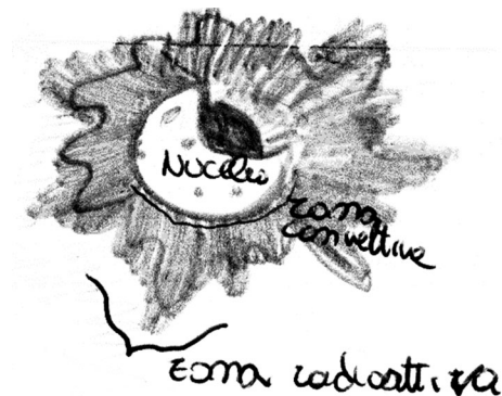
FIG. 5. More precise student sketch of a star's internal and external structure. Translation of Italian labels, from top to bottom: core, convective zone, radiative zone.
