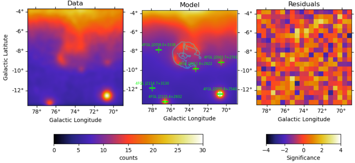
Fig. 2. Maps of a 10^\circ \times 10^\circ region around the Cygnus Loop. Left : count map (pixel size of 0.05^\circ ) smoothed with a Gaussian kernel of 0.2^\circ from 0.1 to 100 GeV. Center : count map expected from the X-ray+UV model (same spatial binning as the left map). Green crosses indicate the positions of \gamma -ray sources listed in the 4FGL catalogue. The cyan line is the contour (10% of the maximum) of the ROSAT X-ray template of the Cygnus Loop (see Sect. 2.2). Right : residual count map from the X-ray+UV template model (pixel size of 0.5^\circ ).
