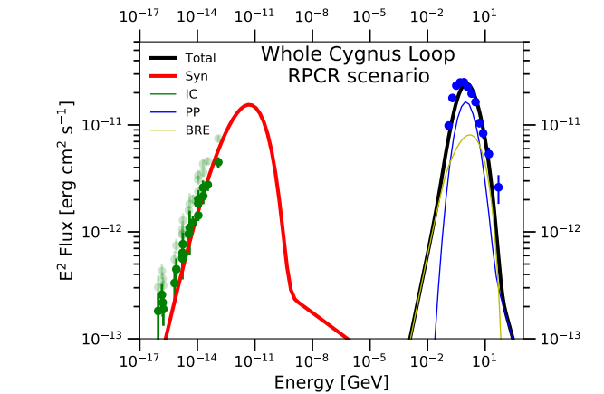
Fig. 11. Radio and \gamma -ray emission from the entire Cygnus Loop. Radio data points (transparent green) from Uyaniker et al. (2004) and Loru et al. (2021) were scaled by a constant factor (dark green) to remove the contribution from the southern region (see Sect. 3.3). The total contribution from Bremsstrahlung, IC, and \pi^0 decay is shown by the solid black line. Upper panel: DSA scenario, adopting values of p_{max}c = 40 GeV, p_{br}c = 62 GeV, W_{tot} = 2.1 \times 10^{49} erg, and K_{ep} = 0.025 for protons and electrons. Lower panel: RPCR scenario, adopting preexisting CR populations from Phan et al. (2018) , s^{1/3}p_{max}c = 20 GeV, s^{1/3}p_{br}c = 70 GeV, and a filling factor f \sim 0.02 .
