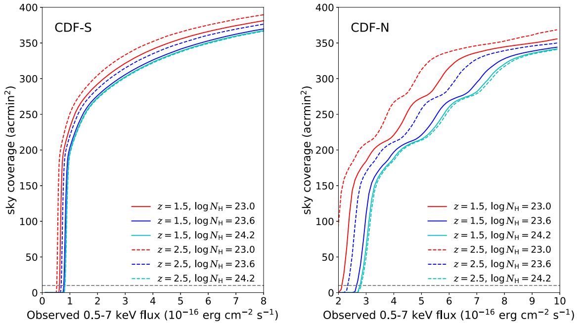
Figure 14. Sky coverage as a function of the observed 0.5–7 keV flux corresponding to the count cut 20 in the CDF-S and CDF-N, shown for three different N_H values at two different redshifts, respectively.
