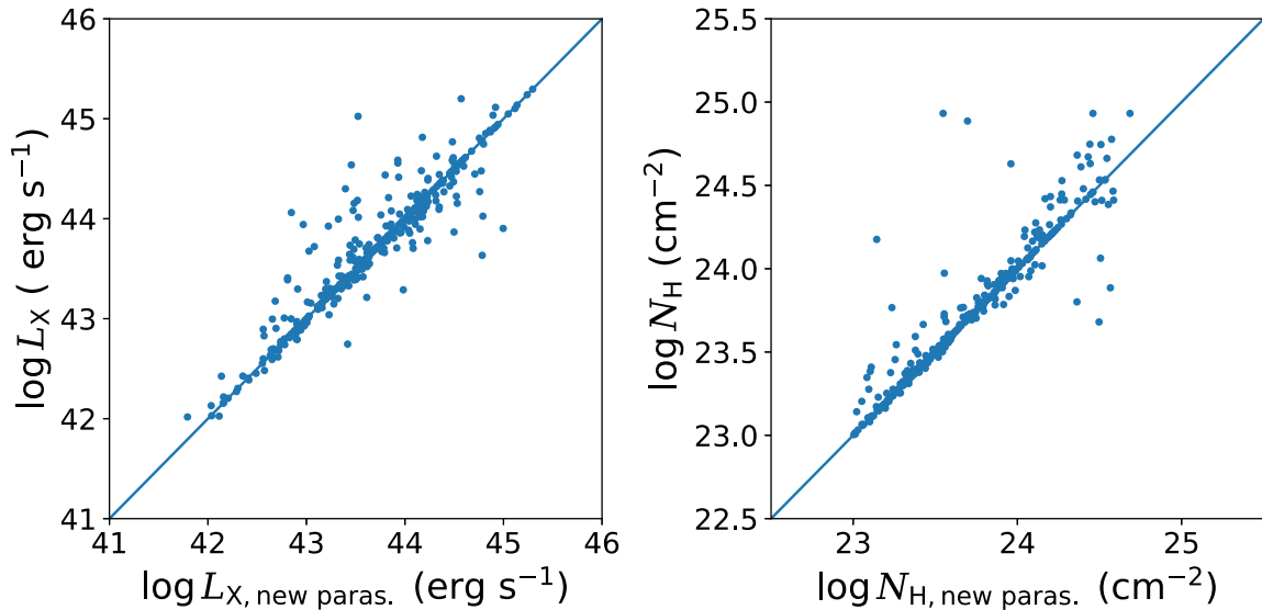
Figure 21. Comparison between the spectral fitting results obtained in Section 3 and those obtained in the Appendix using the new model parameters.
