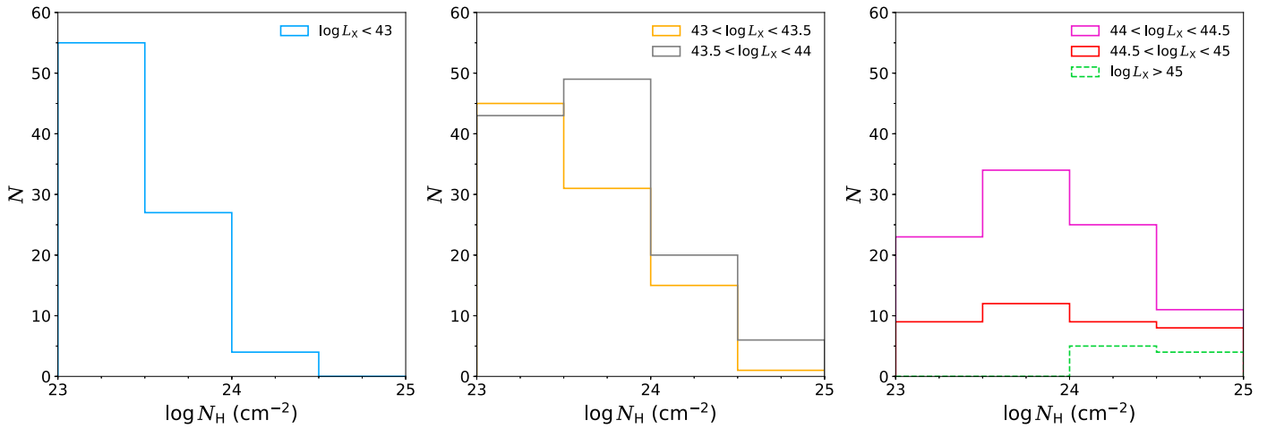
Figure 10. Observed N_H distributions in six L_X bins. The small number of high- N_H sources in low- L_X bins is due to the fact that such sources are difficult to detect. This bias will be corrected in Section 6.4.
