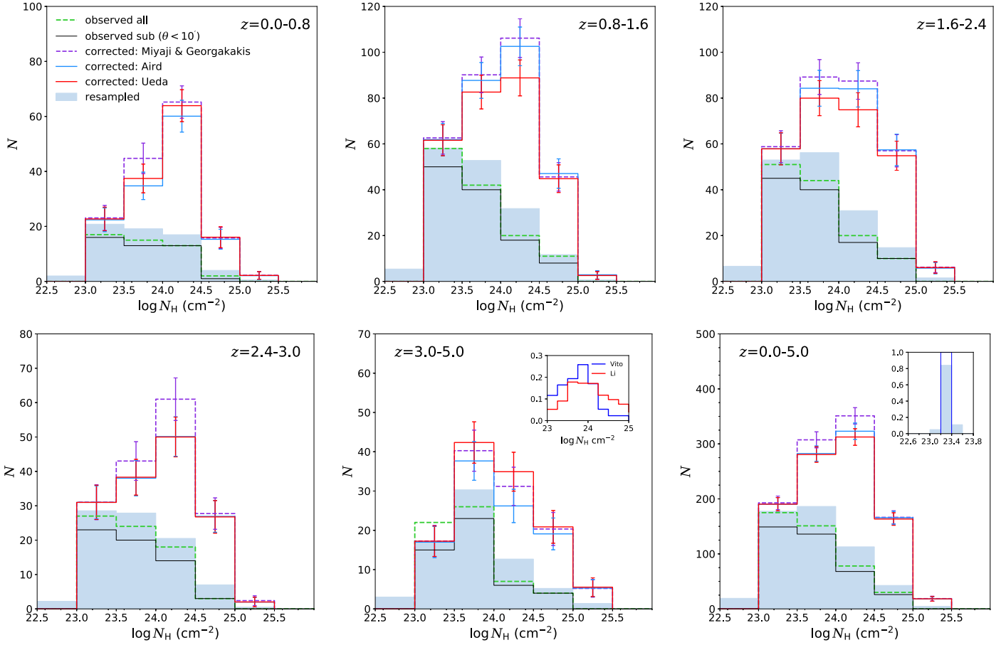
Figure 18. N_H distributions for our HOS in five redshift bins and the entire redshift range ( z = 0-5 ). The error bars are estimated through bootstrapping. In each panel, the green dashed histogram shows the observed best-fit N_H distribution, the black histogram shows the observed N_H distribution for sources with off-axis angle < 10' , the blue shaded area shows the resampled N_H distribution that takes into account the spectral fitting errors and sky coverage effect, and the red and blue solid histograms and purple dashed histogram show the intrinsic N_H distributions after correcting for the undetectable parts of the two surveys using the Ueda et al. (2014), Aird et al. (2015), and Miyaji et al. (2015) and Georgakakis et al. (2015) LFs, respectively. The comparison of the normalized N_H distribution of highly obscured AGNs at z > 3 presented in Vito et al. (2018) and this work is shown in the inset of the z = 3-5 panel; our result shows a systematically higher CT fraction. The inset in the z = 0-5 panel illustrates the effect of the resampling procedure, where the observed N_H distribution shown in blue is resampled into the shaded histogram by considering N_H errors.
