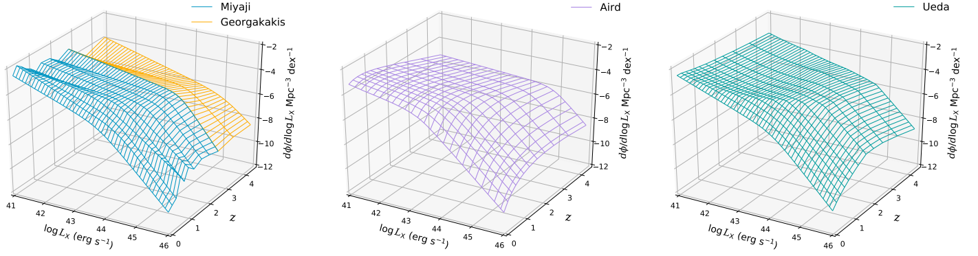
Figure 17. Left: combined X-ray LFs taken from Miyaji et al. (2015) at z < 3 and Georgakakis et al. (2015) at z > 3 . Middle: obscured ( 22 \text{ cm}^{-2} < \log N_H < 24 \text{ cm}^{-2} ) AGN LFs from Aird et al. (2015). Right: Compton-thin AGN ( \log N_H < 24 \text{ cm}^{-2} ) LFs from Ueda et al. (2014).
