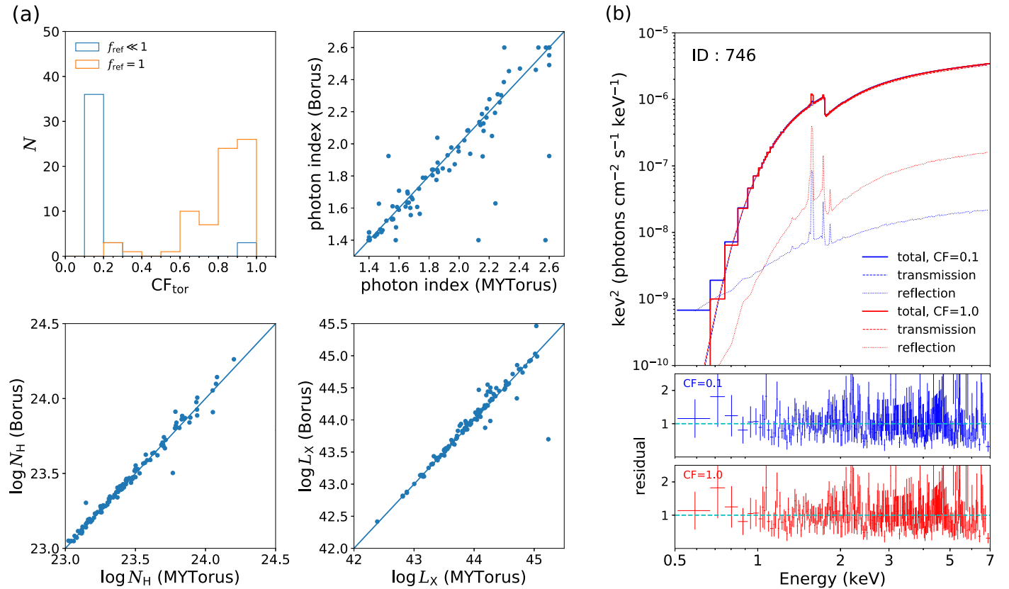
Figure 13. (a) CF derived through the Borus model (Baloković et al. 2018) and the comparisons among photon index, N_H , and L_X obtained from the Borus and MYTorus models. The photon indices in this plot are the original results without fixing \Gamma at 1.8 for some extreme cases. (b) Spectral fitting result for CDF-S XID 746 using the Borus model. Both the fully buried model ( CF_{\text{tor}} = 1.0 ; Cstat = 942.3) and the weak torus model ( CF_{\text{tor}} = 0.1 ; Cstat = 941.8) can well reproduce the data. The contributions from the reprocessed components to the total spectrum in both models are largely weak.
