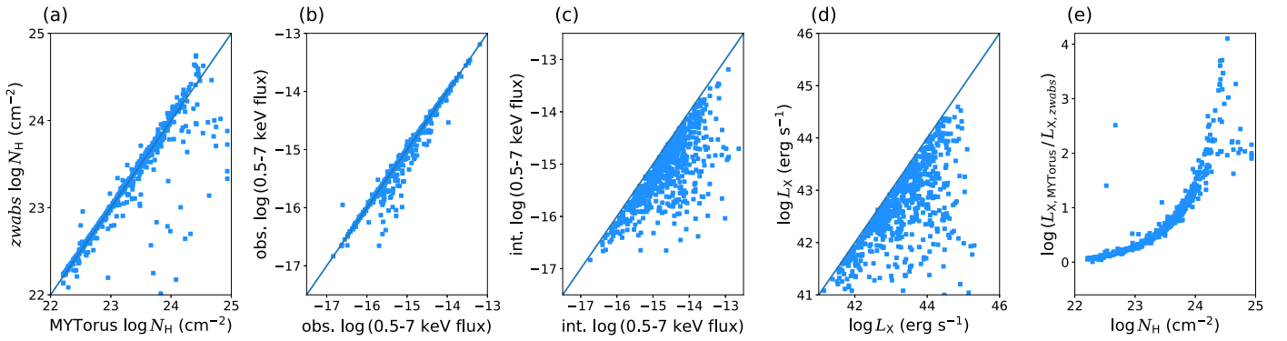
Figure 5. Comparing the spectral fitting results between using the MYTorus (x-axes) and phabs \times zwabs \times zpow (y-axes in all panels but panel (e)) models. (a–d) Comparison results of \log N_H , observed 0.5–7 keV flux, intrinsic 0.5–7 keV flux, and intrinsic 2–10 keV luminosity, respectively. (e) The log-ratio of the intrinsic 2–10 keV luminosity between MYTorus and model z as a function of the MYTorus N_H .
