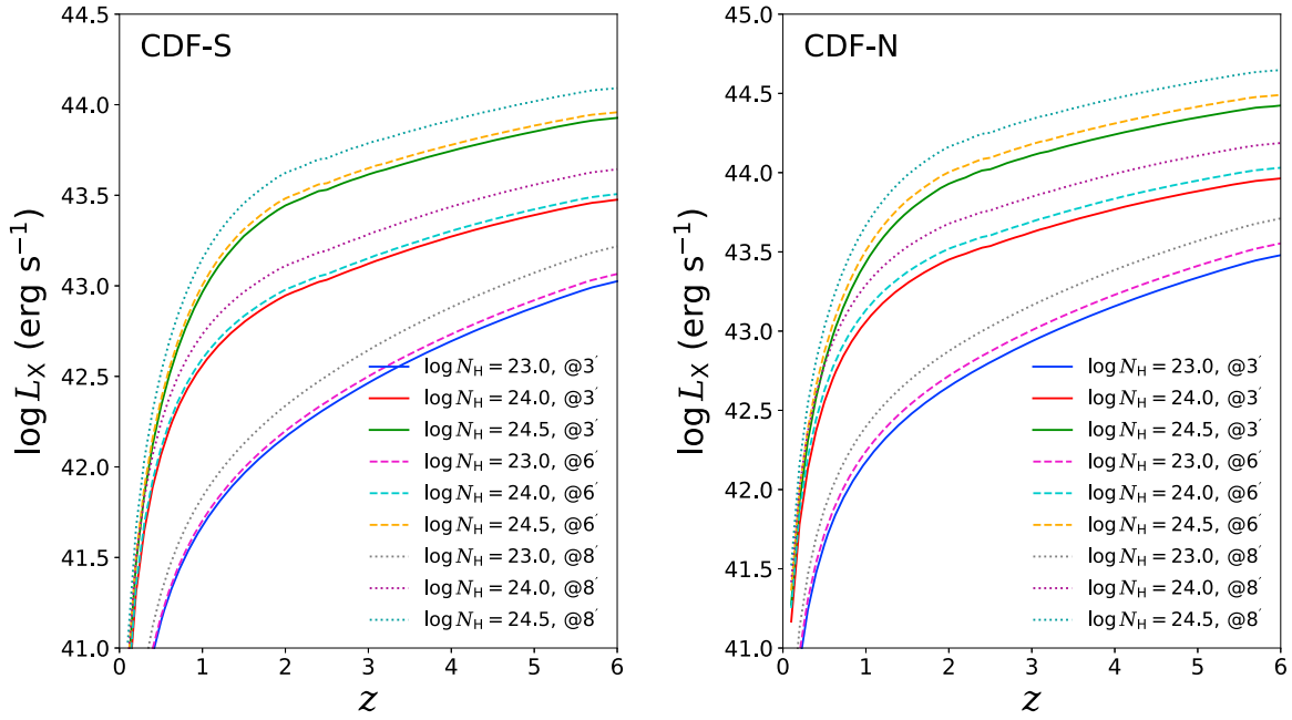
Figure 16. Detection boundary curves as a function of redshift for different N_H and off-axis angles, corresponding to the effective count cut 22.4 in the CDF-S and 21.1 in the CDF-N.
