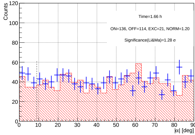
Figure 6. |\mathbf{Alpha}| distributions of the Crab Nebula signal (in blue) and background (in red) estimation from \sim 1.7 hours of ASTRI SST-2M prototype observations taken in December 2017, after an 80% efficiency-based gamma/hadron discrimination parameter cut (in the entire energy range). The region between zero and the vertical dashed line (at 9^\circ ) represents the fiducial signal region. See text for further details.
