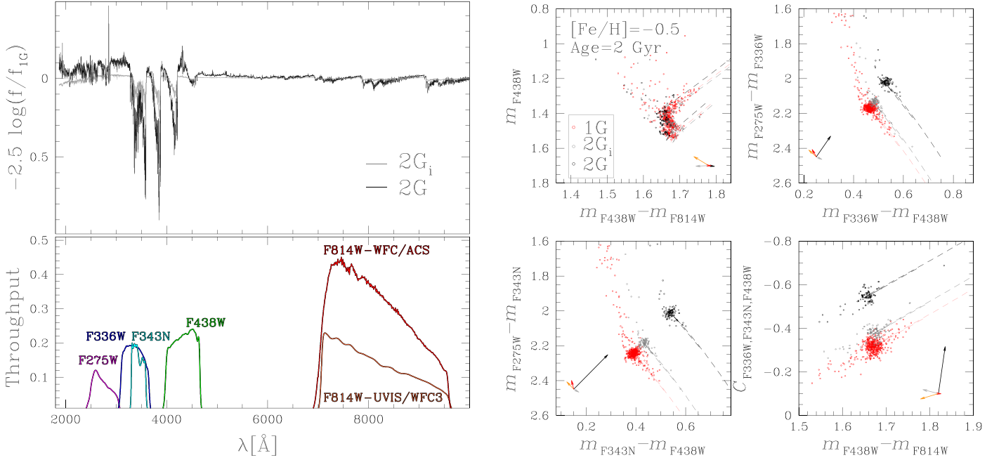
Figure 8. Left panels: flux ratio between the spectrum of 2G (black) or 2G i star (gray) and the spectrum of 1G star with T_{\text{eff}} = 4,898 K and \log g = 2.46 (upper panel). The throughputs of the filters used in this paper are plotted in the bottom panel. Right panels: simulated diagrams of 2 Gyr old HB stars with the same iron abundance, [\text{Fe}/\text{H}] = -0.5 . Red and black dots correspond to 1G and 2G stars, respectively, while gray dots have similar chemical composition to 2G stars of NGC 1978, which are enhanced in nitrogen by 0.1 dex with respect to the 1G. The corresponding isochrones are represented by dashed lines. The gray, black, red, and orange vectors indicate the effect of changing C, N, O, and Fe, respectively, one at a time, on the colors and magnitudes. See text for details.
