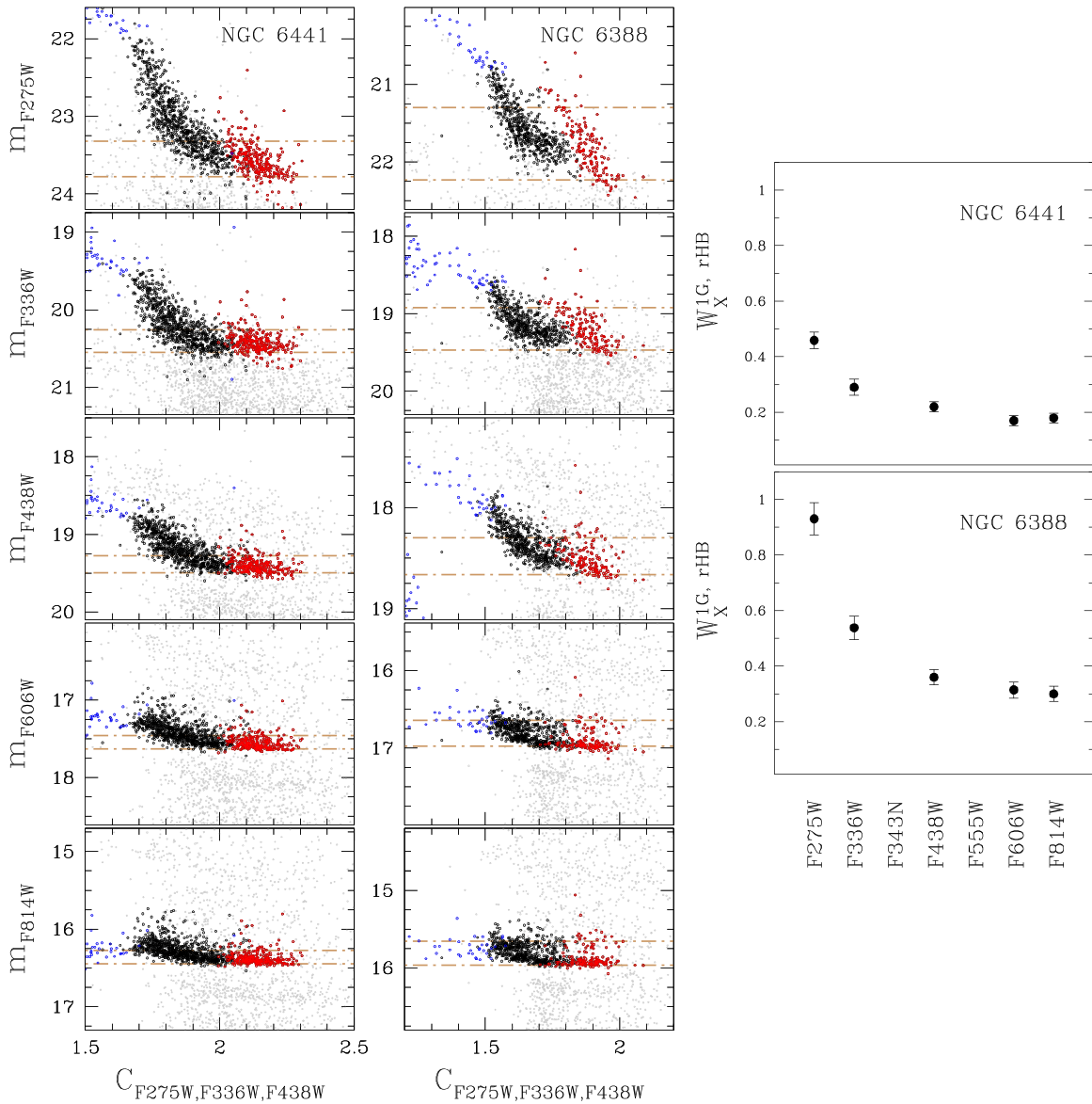
Figure 12. Comparison between the red HBs of NGC 6441 (left panels) and NGC 6388 (middle panels) in the m_X vs. C_{F275W,F336W,F438W} planes, where X = F275W, F336W, F438W, F606W , and F814W . 1G stars, 2G red HB, and 2G blue HB stars are colored red, black, and blue, respectively, while the remaining cluster stars are represented with gray points. The two brown horizontal dotted–dashed lines mark the 10th and 90th percentiles for the magnitude distribution of 1G stars. Right panels show the magnitude extension of 1G stars, W_X^{1G,rHB} , for the available filters.
