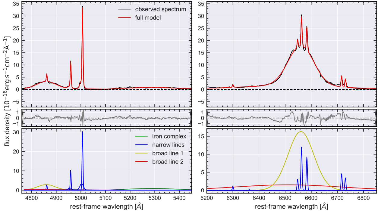
Fig. 4. Fit to the nuclear spectrum of HE 1353–1917 in the wavelength regions around H \beta and H \alpha after continuum subtraction. Upper panels: overlay of the nuclear spectrum (black) and the total fit (red). The residuals from the fit are indicated in gray (offset from the nuclear spectrum for better visibility). Lower panels: individual Gaussian components fitted to the nuclear spectrum together with an Fe II template from Kovačević et al. (2010). All components shown with the same color were kinematically tied to each other during the fit. This includes the narrow components (H \beta_n , [O III] \lambda\lambda 4959 and \lambda 5007, [O I] \lambda 6300 and \lambda 6364, [N II] \lambda 6548 and \lambda 6583, and H \alpha_n and [S II] \lambda\lambda 6717, 6731) shown in blue, the broad components (H \beta_b and H \alpha_b ) shown in yellow, and the very broad components (H \beta_{vb} and H \alpha_{vb} ) shown in red.
