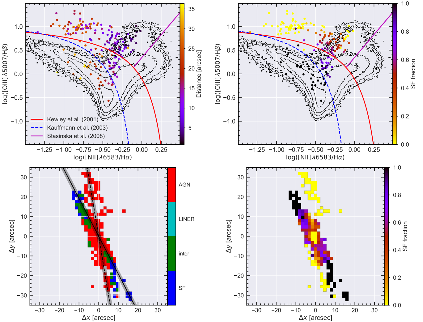
Fig. 7. Top left panel: classical BPT [\text{O III}]/\text{H}\beta vs. [\text{N II}]/\text{H}\alpha diagnostic plot after binning the MUSE data to 1''.2 spatial sampling. The distance from the nucleus is color coded and the distribution of line ratios from the SDSS MPA/JHU catalog is shown as contours for comparison. Demarcation curves from Kauffmann et al. (2003) (dashed blue line), Kewley & Dopita (2002) (red solid line) and Stasińska et al. (2008) (solid magenta line) are displayed for reference. Top right panel: same as the left panel where the color coding represent the SF fraction to the emission line measured as described in the main text. The SF fraction is set to zero for emission regions above the galaxy disc and set to one for regions below the (Kauffmann et al. 2003) demarcation line. Bottom left panel: 2D excitation classification map based on the boundaries set by the demarcation lines. The solid and dashed line represent the primary disc galaxy axis ( \sim 28^\circ with respect to North) and an ENLR axis along ( \sim 10^\circ with respect to North) the strongest emission, respectively. The black shaded area around the axis indicates the 2'' -wide pseudo long-slit extraction region for the metallicity gradients shown in Fig. 8. Bottom right panel: spatial distribution of the SF fraction as defined from the emission-line ratios.
