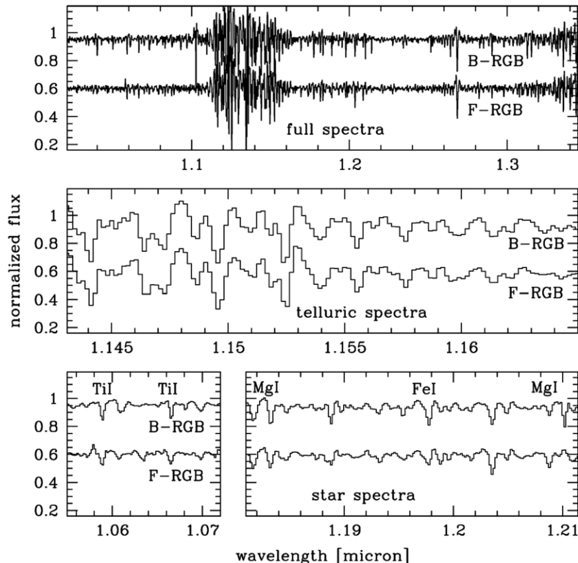
Figure 4. Example of the observed KMOS YJ spectra of two giant stars: a bright B-RGB (star 245899, J = 10.24 mag, top spectra) and a faint F-RGB (star 43138, J = 12.90 mag, bottom spectra). Top panel: observed spectra. Middle panel: zoomed spectra around 1.15 \mu\text{m} , including a few isolated telluric lines. Bottom panel: zoomed spectra around 1.05 and 1.2 \mu\text{m} , including a few isolated stellar features of interest.
