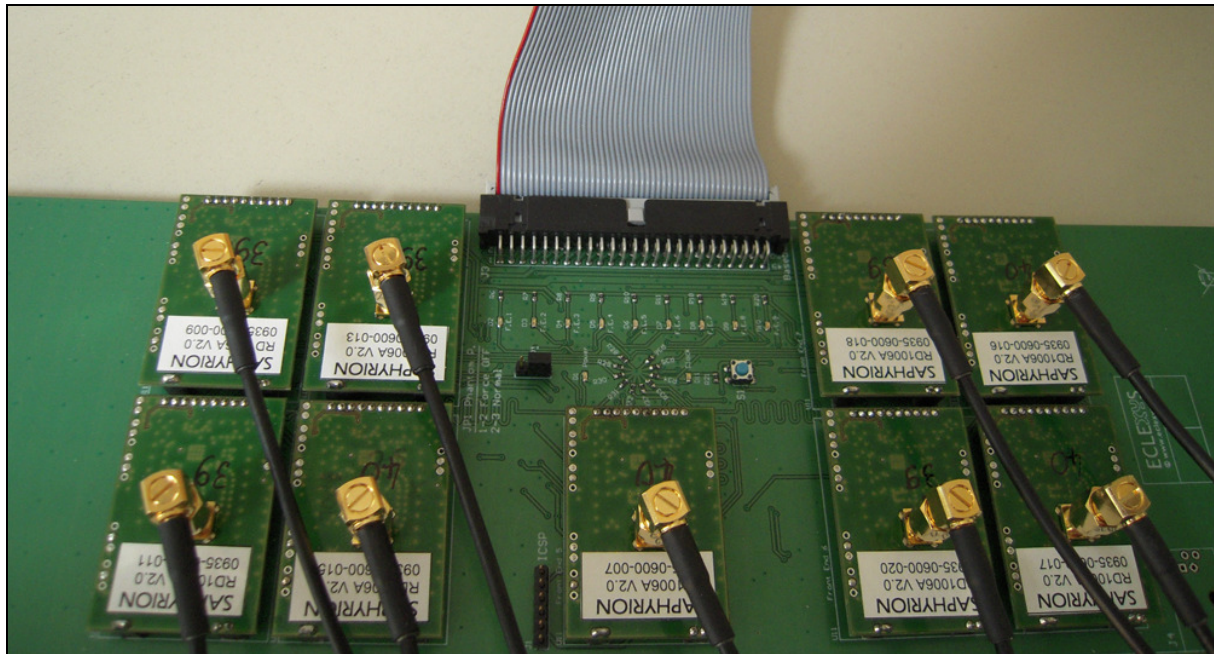
Figure 2.2: Detail of the SM103 module, front-ends
