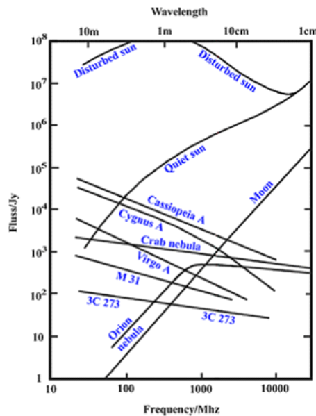
Spectral energy distribution of sky objects in the radio region (from J.D.Kraus)
