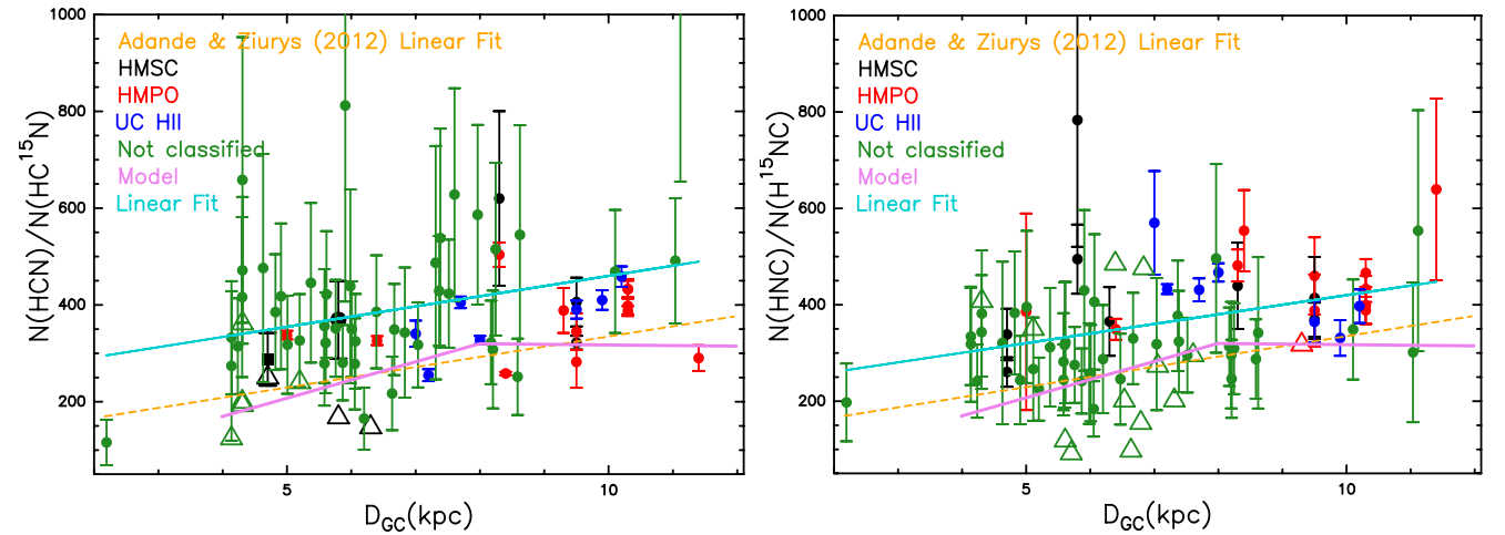
Figure 3. ^{14}\text{N}/^{15}\text{N} ratios for HCN (left panel) and HNC (right panel) as a function of Galactocentric distances of the sources listed in Table 2. Symbols are the same of Fig. 2 but the open triangles are lower limits for the corresponding ^{14}\text{N}/^{15}\text{N} ratio. The cyan solid line is the linear regression fit computed for the two data sets and the pink solid line is the model of Romano et al. (2017). The dashed orange line is the regression linear fit obtained by Adande & Ziurys (2012). Note that we used the scale from 50 to 1000 of y-axes for visualization purposes, and that one source for HCN, with value 1305 \pm 650 , falls outside.
