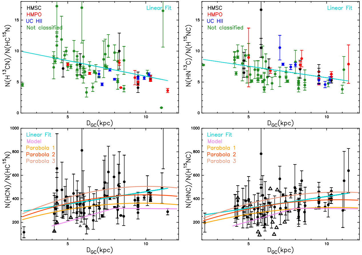
Figure 6. Upper panels: ^{13}\text{C}/^{12}\text{C} and ^{14}\text{N}/^{15}\text{N} ratios for HCN (left panel) and HNC (right panel) as a function of Galactocentric distances of the sources. Symbols are the same as those in Fig. 3 and the cyan solid line is the linear regression fit computed from the two data sets. Note that the negative slope is the consequence of the two combined ratios, ^{13}\text{C}/^{12}\text{C} and ^{14}\text{N}/^{15}\text{N} . Bottom panels: same as in Fig. 3 with all the sources in black, while the three parabolas are described in Section 3.5. The yellow one is found using the minimum value in slope of equation (1) (Parabola 1), the red one is found using the central value of the slope (Parabola 2) and the pink one is found using the maximum value of the slope (Parabola 3). Note that we used the scale from 50 to 1000 of y-axes for visualization purposes, and that one source for HCN, with value 1305 \pm 650 , falls outside.
