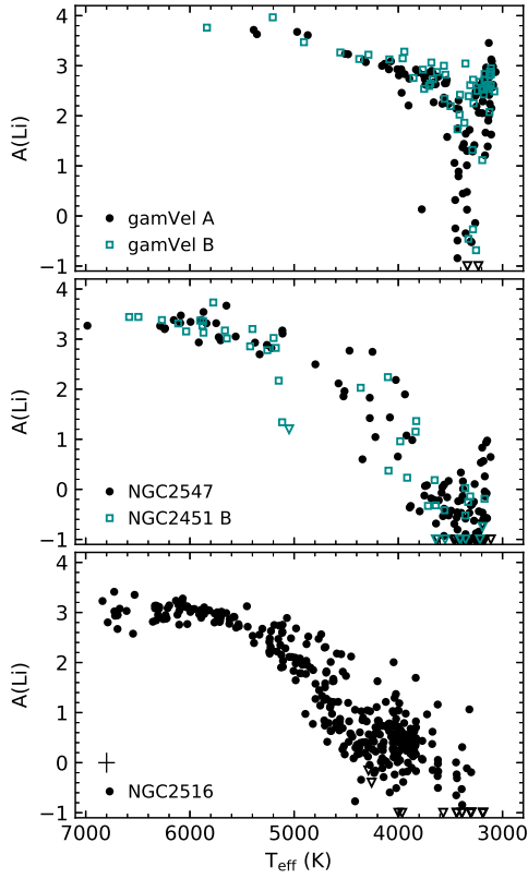
Fig. 1. Evolution of lithium depletion with age: Gamma Vel A and B at \sim 10 – 20 Myr ( top ), NGC 2451 B and NGC 2547 at \sim 35 Myr ( center ), and NGC 2516 at \sim 100 – 140 Myr ( bottom ). Downward triangles indicate upper limits. A typical error bar is shown in the bottom panel.
