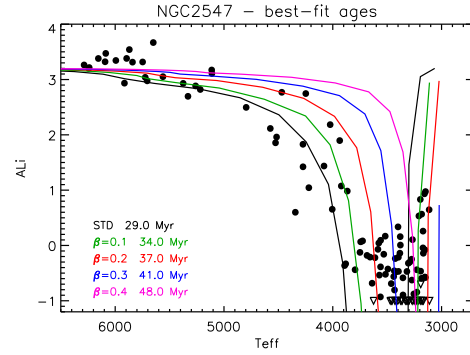
Fig. 3. Comparison of the lithium pattern of NGC 2547 with the predicted isochrones from the standard and spotted models at the ages derived from the best-fits.
