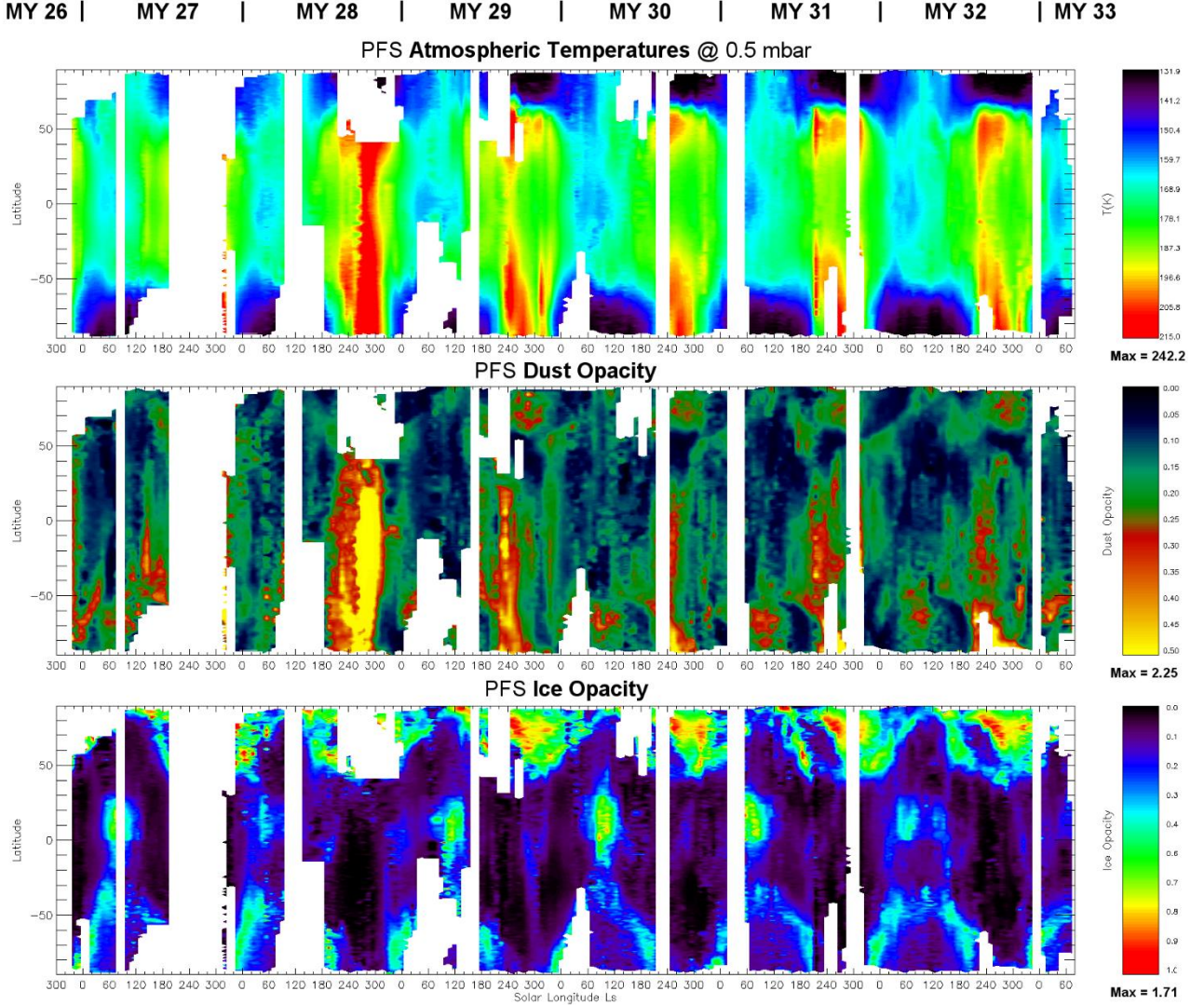
Fig. 1. Zonal-mean atmospheric temperatures at 0.5 mbar (top), integrated dust opacity at 1075 cm -1 (9.3 μm) (middle), and integrated ice opacity at 825 cm -1 (12 μm) (bottom), as a function of latitude and season for different Martian years. The dust opacity is normalized to a reference pressure level of 6.1 mbar.
