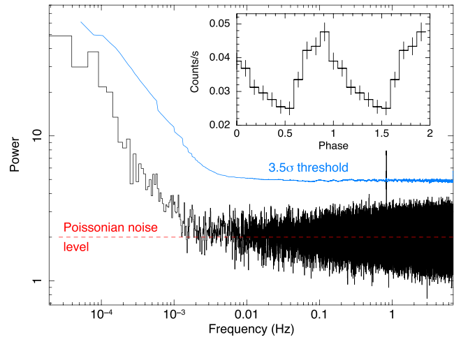
Figure 1. Fourier power spectrum from the 2000 December–2013 February pn data (0.5–10 keV; average of 36 Fourier transforms; \Delta t \approx 73 ms, 262 144 frequencies). The blue line corresponds to the 3.5\sigma confidence level threshold for potential signals and was computed taking into account the number of trials, equal to the number of frequency bins of the spectrum. The prominent peak above the threshold corresponds to the 1.2-s signal. The inset shows the light curve of the data set 0650560301 (where the signal was discovered) folded to its best period.
