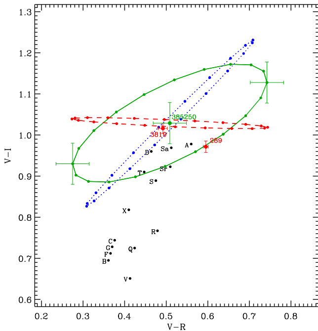
Figure 6. (V - R)/(V - I) colour diagram of the Eureka family member (385250) 2001 DH47 as well as A-class asteroids (289) Nenetta and (3819) Robinson versus mean colours of the different taxonomic classes discussed in the text. The three ellipses shown in the plot represent the systematic uncertainty in the colours of (385250) 2001 DH47 due to the light-curve effect. These are shown for the rotation period solution ( P = 4 h; green line), as well as for two extreme cases: P = 3.2 h (blue dotted line) and P = 4.8 h (red dashed line). If our measurements were free from the random error, our estimated colours for this asteroid should be located on one of the ellipses. Note that the random uncertainties (shown by error bars) are smaller than this systematic effect.
