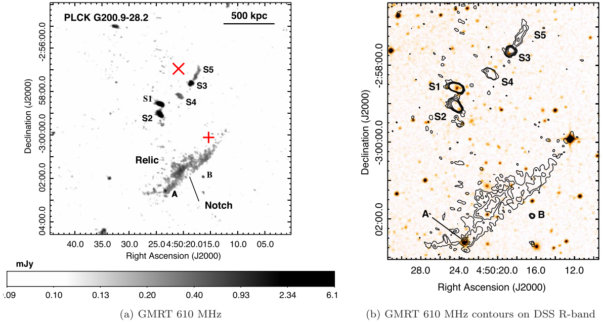
Figure 1. (a) GMRT 610 MHz image is shown in grey-scale. The 610 MHz image has a resolution of 5.6 \text{ arcsec} \times 4.7 \text{ arcsec} , position angle 59^\circ.4 and rms noise, \sigma_{\text{rms}} = 0.045 \text{ mJy beam}^{-1} . The discrete sources in the central region are labelled S1–S5 and those near the extended source labelled ‘Relic’ are A and B. The symbols ‘x’ and ‘+’ mark the positions of the cluster according to the XMM-Newton and the Planck measurements, respectively. (b) Digitized Sky Survey R -band image of the region of the labelled sources is shown in grey-scale with the GMRT 610 MHz contours overlaid. The contour levels are 3\sigma_{\text{rms}} \times [\pm 1, 2, 4, \dots] mJy beam -1 .
