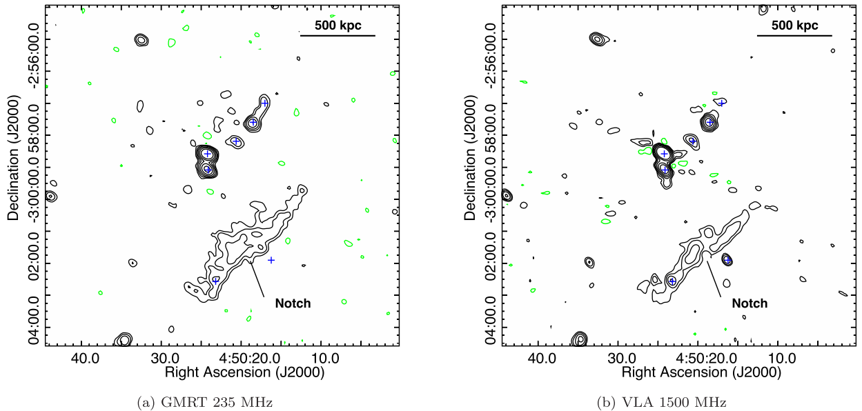
Figure 2. (a) GMRT 235 MHz image with \sigma_{\text{rms}} = 0.39 \text{ mJy beam}^{-1} and resolution of 14.7 \text{ arcsec} \times 12.8 \text{ arcsec} , position angle 57^\circ.6 is shown in contours. (b) VLA 1.5 GHz image with a resolution of 14.5 \text{ arcsec} \times 10.0 \text{ arcsec} , position angle 33^\circ.7 and \sigma_{\text{rms}} = 0.06 \text{ mJy beam}^{-1} is shown in contours. In panels a and b, the black are positive and the green are negative contour levels. The plus signs mark the discrete sources labelled in Fig. 1.
