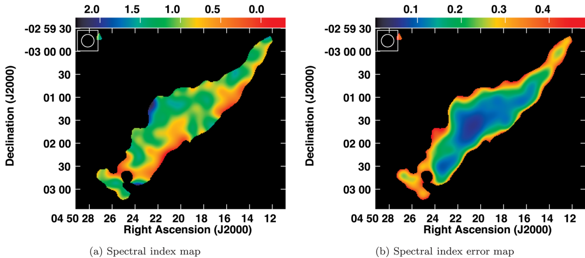
Figure 5. (a) The spectral index map of the radio relic between 235 and 610 MHz. (b) The corresponding noise map. The resolution of the maps shown in upper left corner of each panel is 16.4 arcsec \times 16.4 arcsec.
