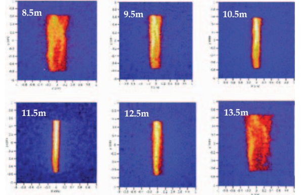
Fig. 4. Diffracted images at 150 keV at several distances between the GaAs crystal and the focal plane imager. The width of the diffracted image in the focusing direction reaches the minimum (best focusing) at 11.5 m rather than at the focal length of 20 m, due to the divergence of the X-ray beam at 22 m from the Laue lens support.
