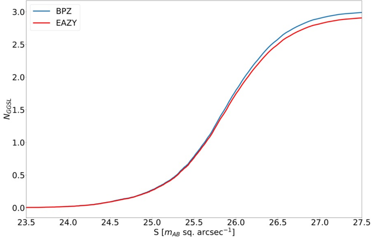
Figure S6: Expected number of GGSL events in the field of MACS1206. The number is calculated using Eq. S9 , assuming the source number density n(S, z) as measured in the HUDF, based on photometric redshift catalogs (16). The blue and the red lines show the results based on the photometric redshift estimates obtained with two different codes, namely BPZ (109) and EAZY (110). The estimated number of events is shown as a function of the minimal source surface brightness.
