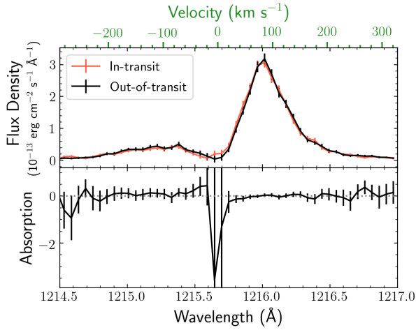
Figure 6. Top. \text{Ly}\alpha line of GJ 9827 during the transit (red line) and outside (black line). Bottom. In-transit absorption depth, 1 - F_{\text{IN}}/F_{\text{OUT}} .
