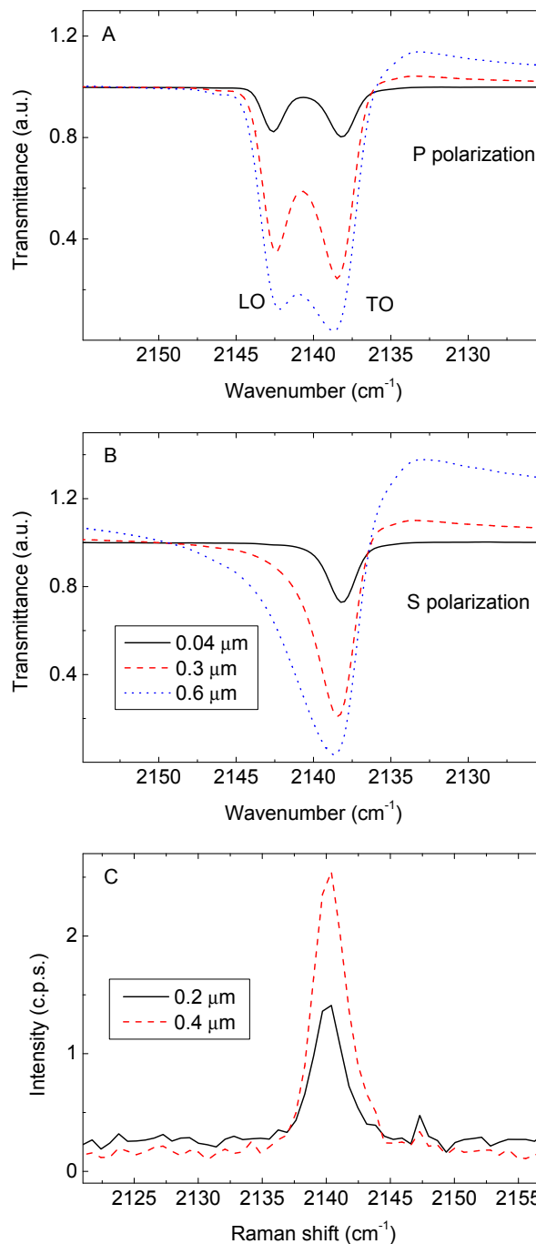
Fig. 7. Thickness experiment. Panel A): IR spectra in P polarization; panel B): IR spectra in S polarization. CO film thickness: black solid line: 0.04 \mu m ; red dashed line: 0.3 \mu m ; blue dotted line: 0.6 \mu m . Panel C): Raman experiment. CO stretching mode band of a 0.2 \mu m (black solid line) and 0.4 \mu m (red dashed line) film.
