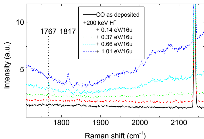
Fig. 6. Raman spectra of solid CO irradiated with 200 keV H^+ . CO film as deposited (black solid line); CO film after irradiation dose of 0.14 eV/16u (red dashed line), 0.37 eV/16u (green dotted line), 0.66 eV/16u (cyan short-dashed line), and 1.01 eV/16u (blue dash-dotted line). Black dotted vertical lines indicate 1767 cm^{-1} unidentified band and 1817 cm^{-1} band tentatively attribute to C_2 .
