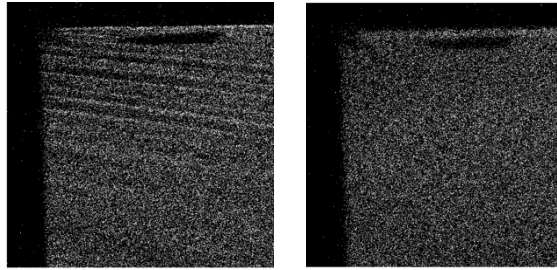
Figure 7. Improvement in the uniformity by dithering of the BE: no oscillation (left), oscillation with range = 0.5 mm and period = 20 s (right). The images are taken with exposure of 30min.
