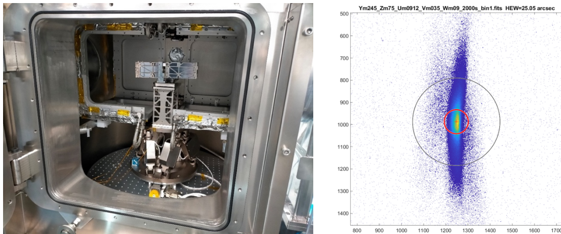
Figure 9. Left: MM-0042 installed in the experimental chamber of BEatriX. Right: acquired image of MM-0042; the two circles correspond to HEW (red) and 90% EE (black).
