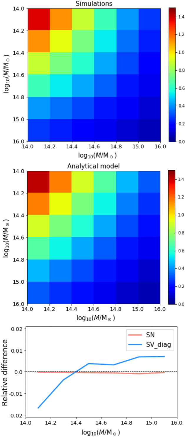
Fig. A.1. Normalized sample covariance between mass bins from simulations (top) and our analytical model (center), computed for 10^6 spherical sub-boxes of radius R = 200 h^{-1} \text{ Mpc} at redshift z = 0.506 and in the mass range of 10^{14} \leq M/M_{\odot} \leq 10^{16} . Bottom panel: relative difference between simulations and model for the diagonal elements of the sample covariance matrix (blue) and for the shot-noise (red).
