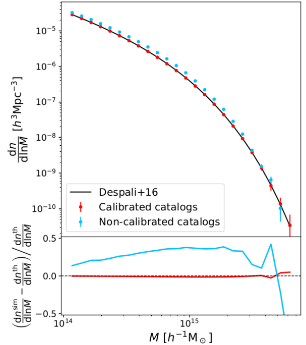
Fig. 1. Halo mass function for the mass calibration of the PINOCCHIO catalogs. Top panel: comparison between the mass function from the calibrated (red) and the non-calibrated (blue) light cones, averaged over the 1000 catalogs, in the redshift bin z = 0.1 – 0.2 . Error bars represent the standard error on the mean. The black line is the D16 mass function. Bottom panel: relative difference between the mass function from simulations and that of D16.
