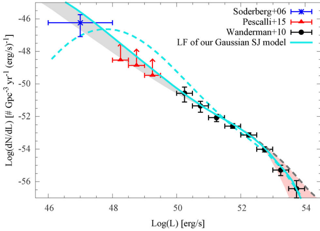
Figure 6. The light blue line represents the LF of our fiducial model (see Table 1). There are two shaded areas obtained by varying one parameter and leaving the others fixed: the grey one refers to 1 \leq \theta_\Gamma/\theta_c \leq \sqrt{2} , while the pink one refers to \sigma = \sqrt{\sigma_{\log t}^2 + \sigma_{\log \epsilon_c}^2} between 0.35 and 0.78 dex. The dashed grey line (visible on the bottom-right corner) is the LF for \theta_c = 5^\circ , while the dashed light blue line is the LF for \theta_\Gamma/\theta_c = 0.5 , both with all other parameters fixed. The data points are the same as in Pescalli et al. (2015), and are partly based on previous works by Soderberg et al. (2006) and Wanderman & Piran (2010). Red points are lower limits.
