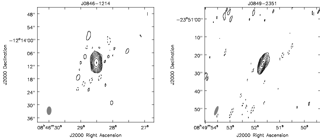
Figure B.14. left panel: J0846-1214, rms = 13 \mu\text{Jy beam}^{-1} , contour levels at -3, 3 \times 2^n , n \in [0,7] , beam size 9.14 \times 4.93 kpc. right panel: J0849-2351, rms = 6 \mu\text{Jy beam}^{-1} , contour levels at -3, 3 \times 2^n , n \in [0,5] , beam size 15.29 \times 4.36 kpc.
