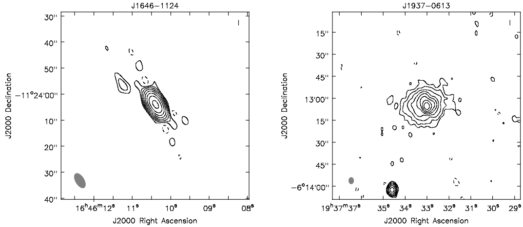
Figure B.23. left panel: J1646-1124, rms = 22 \mu\text{Jy beam}^{-1} , contour levels at -3, 3 \times 2^n , n \in [0,7] , beam size 10.09 \times 5.26 kpc. right panel: J1937-0613, rms = 9 \mu\text{Jy beam}^{-1} , contour levels at -3, 3 \times 2^n , n \in [0,7] , beam size 0.95 \times 0.72 kpc.
