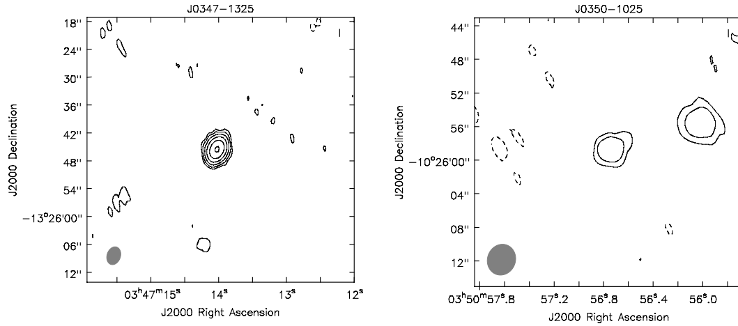
Figure B.6. left panel: J0347-1325, rms = 6 \mu\text{Jy beam}^{-1} , contour levels at -3, 3 \times 2^n , n \in [0, 5] , beam size 17.82 \times 13.10 kpc. right panel: J0350-1025, rms = 5 \mu\text{Jy beam}^{-1} , contour levels at -3, 3 \times 2^n , n \in [0, 1] , beam size 10.83 \times 9.72 kpc.
