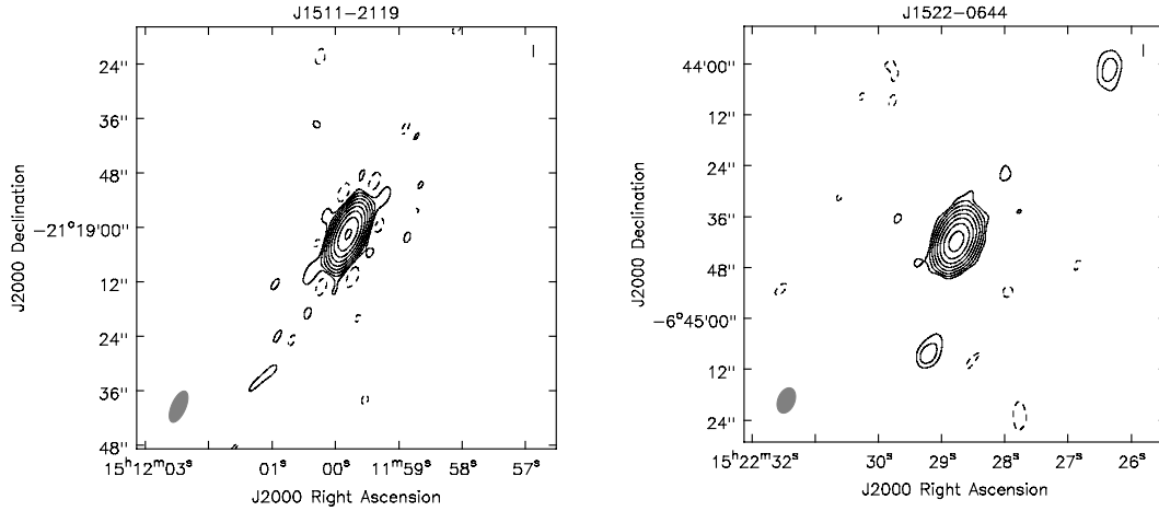
Figure B.20. left panel: J1511–2119, rms = 21 \mu\text{Jy beam}^{-1} , contour levels at -3, 3 \times 2^n , n \in [0,8] , beam size 7.07 \times 3.02 kpc. right panel: J1522–0644, rms = 8 \mu\text{Jy beam}^{-1} , contour levels at -3, 3 \times 2^n , n \in [0,7] , beam size 11.46 \times 7.32 kpc.
