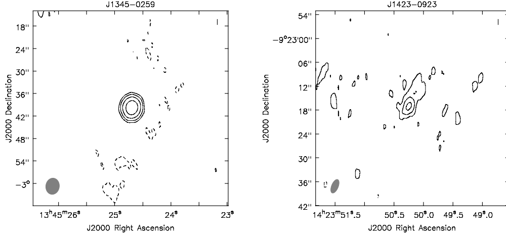
Figure B.19. left panel: J1345–0259, rms = 9 \mu\text{Jy beam}^{-1} , contour levels at -3, 3 \times 2^n , n \in [0,3] , beam size 8.20 \times 6.78 kpc. right panel: J1423–0923, rms = 6 \mu\text{Jy beam}^{-1} , contour levels at -3, 3 \times 2^n , n \in [0,2] , beam size 5.42 \times 2.50 kpc.
