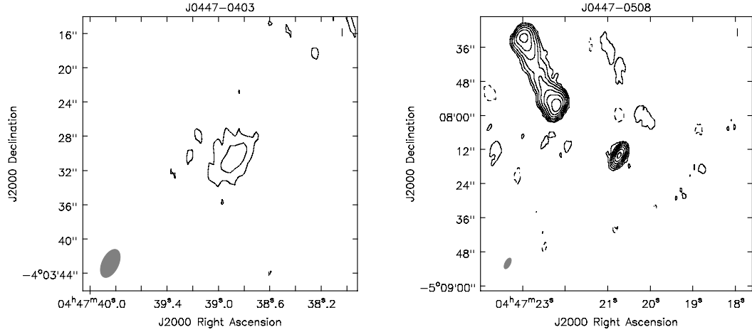
Figure B.10. left panel: J0447-0403, rms = 5 \mu\text{Jy beam}^{-1} , contour levels at -3, 3 \times 2^n , n \in [0,1] , beam size 3.39 \times 1.84 kpc. right panel: J0447-0508, rms = 15 \mu\text{Jy beam}^{-1} , contour levels at -3, 3 \times 2^n , n \in [0,6] , beam size 7.44 \times 3.39 kpc.
