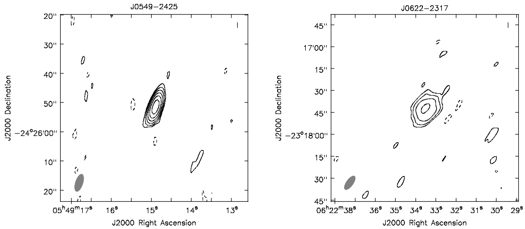
Figure B.12. left panel: J0549-2425, rms = 10 \mu\text{Jy beam}^{-1} , contour levels at -3, 3 \times 2^n , n \in [0,5] , beam size 5.95 \times 2.43 kpc. right panel: J0622-2317, rms = 10 \mu\text{Jy beam}^{-1} , contour levels at -3, 3 \times 2^n , n \in [0,3] , beam size 8.89 \times 3.67 kpc.
