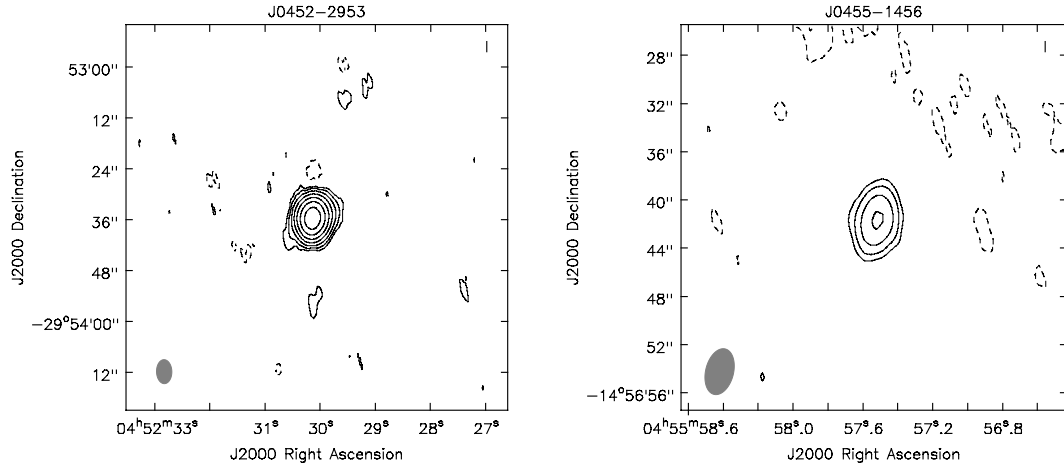
Figure B.11. left panel: J0452-2953, rms = 8 \mu\text{Jy beam}^{-1} , contour levels at -3, 3 \times 2^n , n \in [0,6] , beam size 40.37 \times 25.70 kpc. right panel: J0455-1456, rms = 5 \mu\text{Jy beam}^{-1} , contour levels at -3, 3 \times 2^n , n \in [0,3] , beam size 12.13 \times 7.22 kpc.
