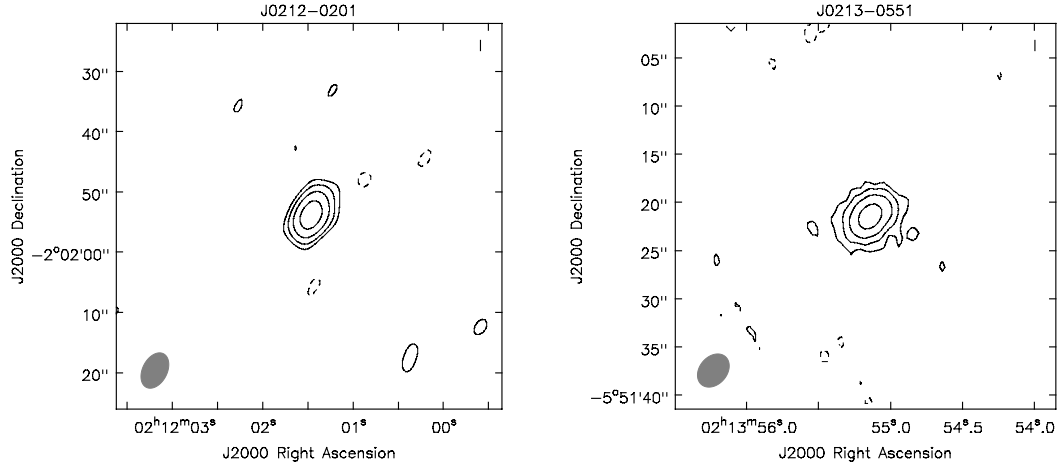
Figure B.4. left panel: J0212-0201, rms = 6 \mu\text{Jy beam}^{-1} , contour levels at -3, 3 \times 2^n , n \in [0, 3] , beam size 73.33 \times 47.79 kpc. right panel: J0213-0551, rms = 5 \mu\text{Jy beam}^{-1} , contour levels at -3, 3 \times 2^n , n \in [0, 3] , beam size 12.24 \times 9.13 kpc.
