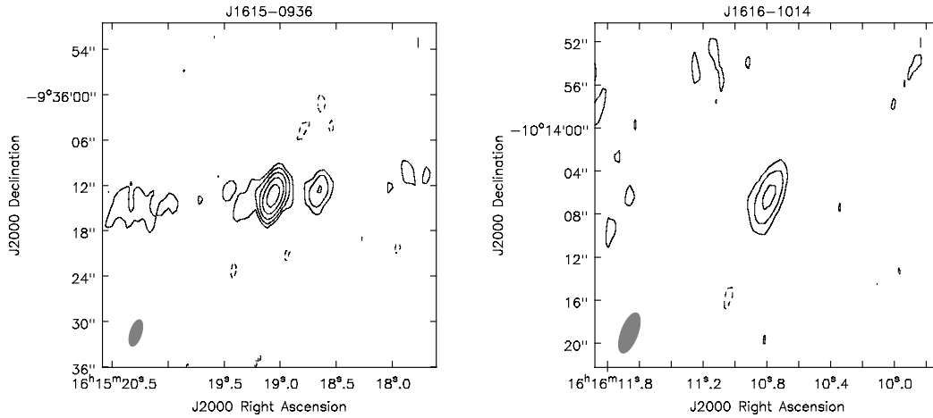
Figure B.21. left panel: J1615–0936, rms = 7 \mu\text{Jy beam}^{-1} , contour levels at -3, 3 \times 2^n , n \in [0,4] , beam size 5.17 \times 2.17 kpc. right panel: J1616–1014, rms = 5 \mu\text{Jy beam}^{-1} , contour levels at -3, 3 \times 2^n , n \in [0,2] , beam size 6.73 \times 2.66 kpc.
