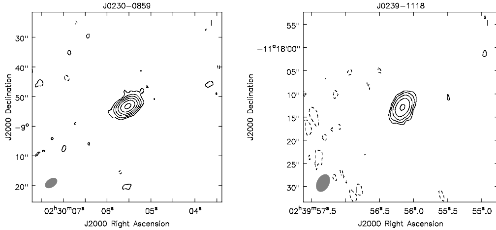
Figure B.5. left panel: J0230-0859, rms = 9 \mu\text{Jy beam}^{-1} , contour levels at -3, 3 \times 2^n , n \in [0, 5] , beam size 1.50 \times 0.92 kpc. right panel: J0239-1118, rms = 6 \mu\text{Jy beam}^{-1} , contour levels at -3, 3 \times 2^n , n \in [0, 4] , beam size 19.13 \times 12.45 kpc.
