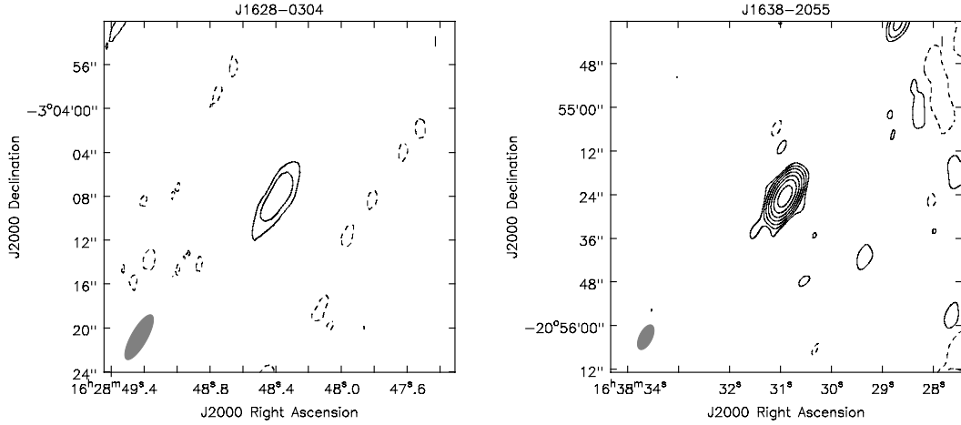
Figure B.22. left panel: J1628-0304, rms = 6 \mu\text{Jy beam}^{-1} , contour levels at -3, 3 \times 2^n , n \in [0,1] , beam size 9.58 \times 2.99 kpc. right panel: J1638-2055, rms = 11 \mu\text{Jy beam}^{-1} , contour levels at -3, 3 \times 2^n , n \in [0,6] , beam size 4.22 \times 2.01 kpc.
