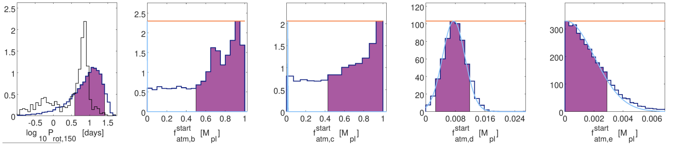
Figure 14. From left to right: Posterior distributions (dark blue lines) of the stellar rotation period at an age of 150 Myr and of the initial atmospheric mass fractions of TOI-561 b, c, d and e. In each panel, the purple region represents the 68 per cent highest probability density intervals. In the left panel, the black thin line shows the rotation period distribution of stars member of open clusters with ages around 150 Myr. Data are taken from Johnstone et al. (2015a) , who report the rotation period of \sim 2000 stars belonging to the Pleiades, M50, M35, and NGC 2516, whose ages are between 125 and 150 Myr. To generate the black histogram we selected a sub-sample of 578 stars, which have masses that deviate from M_\star less than 0.1 M_\odot . In the other panels, the horizontal orange lines mark the uniform prior used in the fit, scaled to the highest peak of each posterior distribution for better visualization. The light blue lines indicate the current atmospheric mass fraction of each planet determined as described in Section 6.
