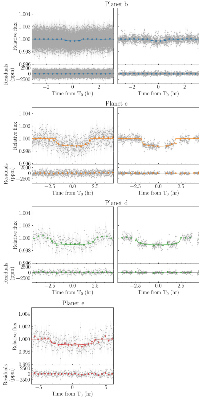
Figure 8. Phase-folded TESS (left) and CHEOPS (right) light curves of TOI-561 b, c, and d. Planet e shows a single transit in the TESS light curve, and it has no CHEOPS observations. For each planet, the coloured line indicates the best-fitting model, and residuals are shown in the bottom panels. Data points binned over 20 min (planet b) and 30 min (planets c, d and e) are shown with coloured dots.
