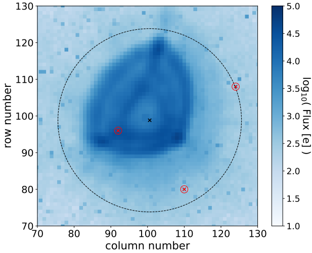
Figure 2. Extraction of 60 \times 60 arcsec of the CHEOPS FoV during the third visit centered on TOI-561. The dashed black circle represents the RINF photometric aperture surrounding the CHEOPS PSF, whose centroid is marked by the black cross. The positions of the three identified telegraphic pixels, including the one located within the CHEOPS PSF (see Appendix A), are highlighted by the red, circled crosses.
