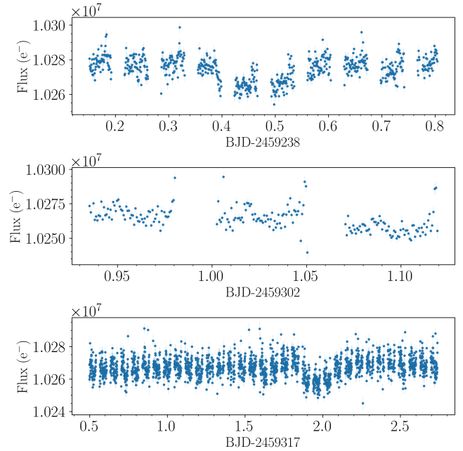
Figure A1. CHEOPS RINF light curves of TOI-561 as extracted from the DRP, with 4\sigma -clipping for outliers removal. Visits 1, 2 and 3 are shown from top to bottom.
