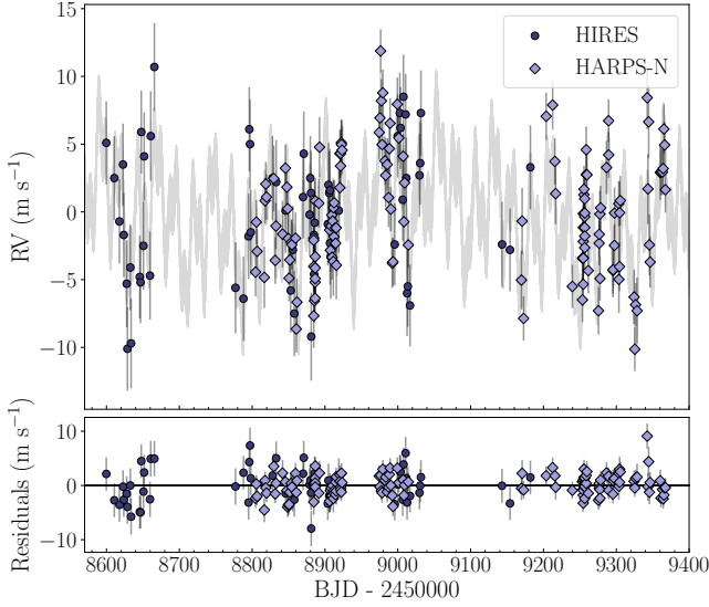
Figure 10. Global model (grey line) with residuals of HARPS-N and HIRES RVs according to the 5-Keplerian photometric and spectroscopic fit. The error bars include the jitter term added in quadrature.
