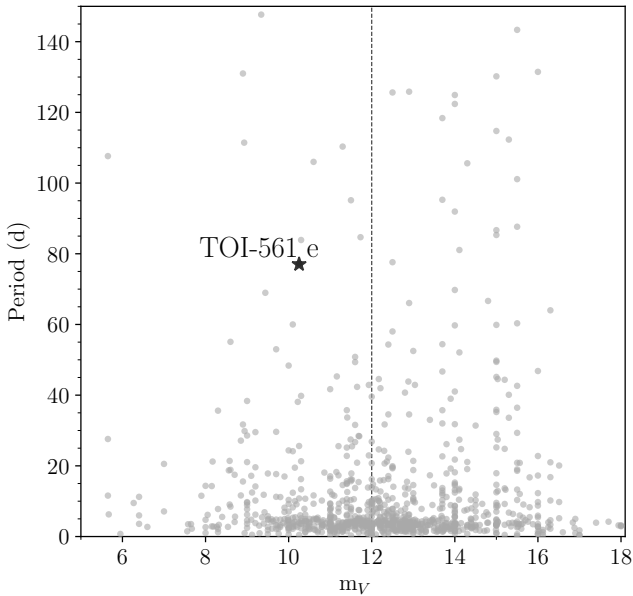
Figure 15. V magnitude versus planetary periods for confirmed transiting exoplanets as reported in the Extrasolar Planets Encyclopaedia catalogue ( http://exoplanet.eu/catalog/ ) in date 18 October 2021. The dashed vertical line marks V = 12 mag. TOI-561 e is one of the few long-period planets orbiting a star bright enough for precise RV characterization.
