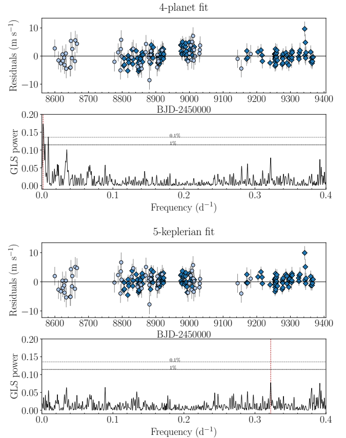
Figure 6. Time series and GLS periodogram of the RV residuals after the 4-planet and 5-Keplerian fits as described in Section 4.2. In the residuals plot, the HARPS-N and HIRES RVs are plotted with dark blue diamonds and light blue circles, respectively. In the periodogram plots, the dashed and dotted horizontal lines show the 1 and 0.1 per cent False Alarm Probability (FAP) level, respectively. The red vertical line indicates the main peak of each periodogram. The long-period peak around frequencies 0.0017 - 0.0025 \text{ d}^{-1} ( P = 400 - 600 \text{ d} ) in the 4-planet residuals periodogram is modelled by the fifth Keplerian, and no more significant peaks are identified in the 5-Keplerian residuals periodogram. Moreover, the positive variation at \sim 9000 BJD–2450000 in the 4-planet fit residuals disappears in the 5-Keplerian fit residuals.
