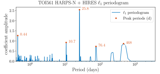
Figure 5. \ell_1 -periodogram of the combined HARPS-N and HIRES data sets, computed on a grid of frequencies from 0 to 2.5 cycles per day. The total time-span of the observations is 768 days. The code automatically accounts for the offset between HARPS-N and HIRES data by using the mean value of each data set.
