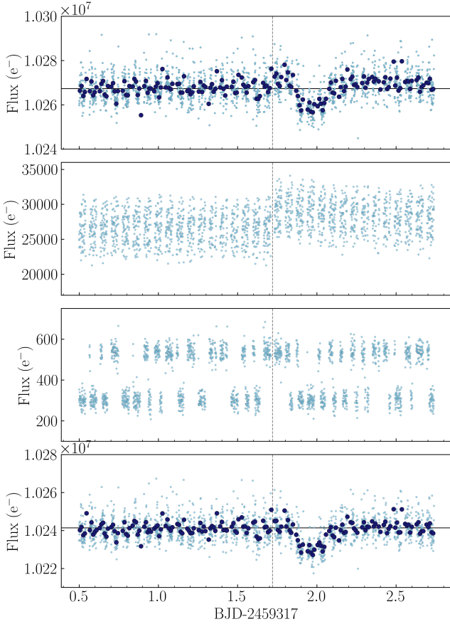
Figure A2. Top panel: TOI-561 RINF original light curve of the third visit (light blue dots) after the removal of 4\sigma outliers, with over-plotted the 15-minute binned light curve (dark blue dots). The start of the flux jump due to the telegraphic pixel is marked with the dashed vertical line. Second panel: light curve of the telegraphic pixel located within the CHEOPS PSF. Third panel: light curve of the two additional telegraphic pixels located within the RINF aperture. Bottom panel: corrected light curve after masking the three telegraphic pixels.
