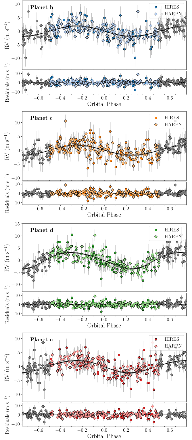
Figure 9. Phase-folded HARPS-N and HIRES RVs with residuals of TOI-561 b, c, d and e, as resulting from the joint photometric and spectroscopic fit. The error bars include the jitter term added in quadrature.
