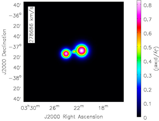
Figure 6. Fornax A model image at \nu = 100 MHz (from McKinley et al. 2015). Units are Jy pixel ^{-1} with a pixel size = 0.75 arcmin.
