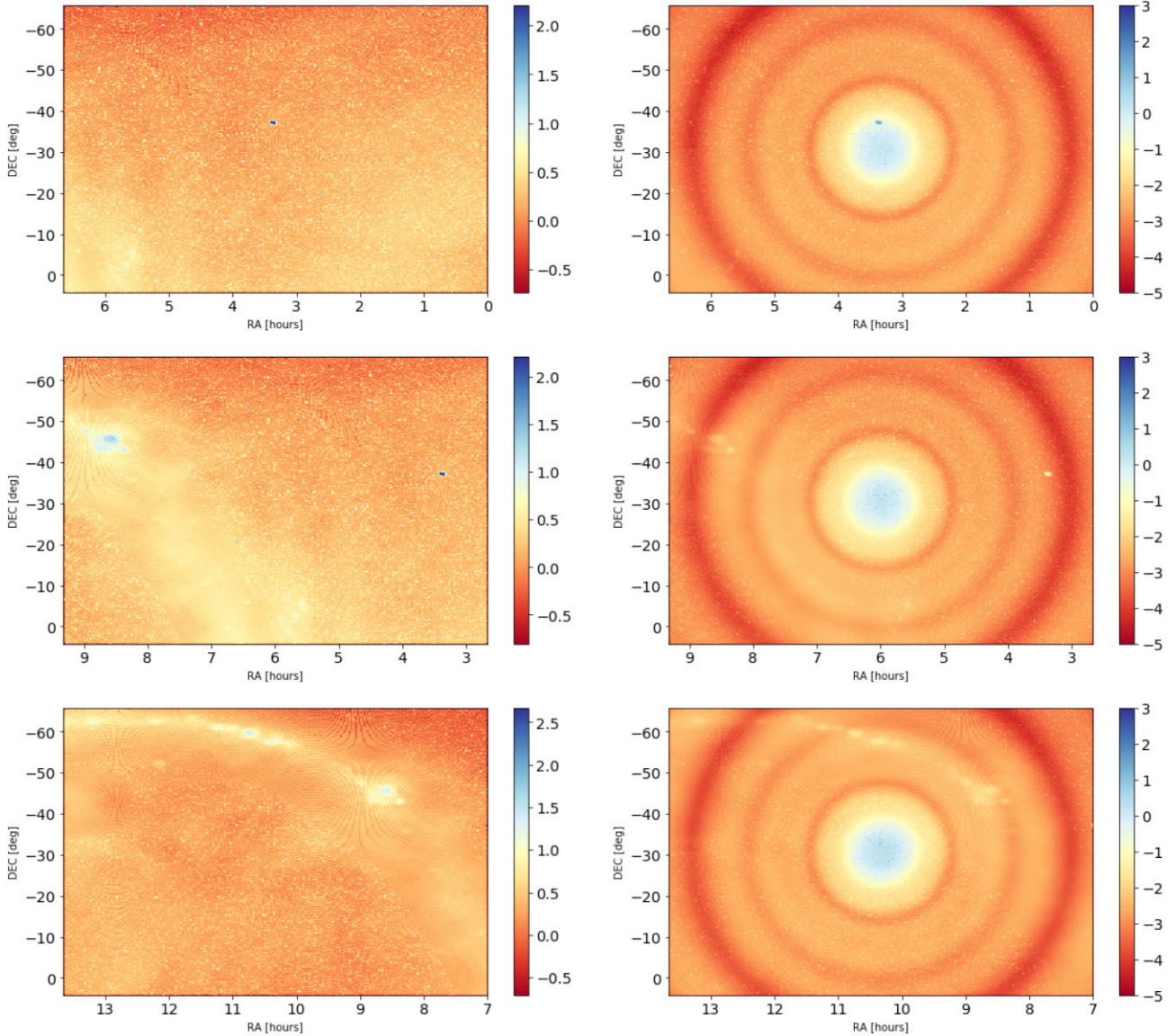
Figure 7. Left-hand column shows sky model images of simulated fields, field 1 (first row), field 2 (second row), and field 3 (third row). Right-hand column shows the corresponding apparent sky model, i.e. after the primary beam, E_H is applied. Units are \log_{10}[I(\text{Jy pixel}^{-1})] .
