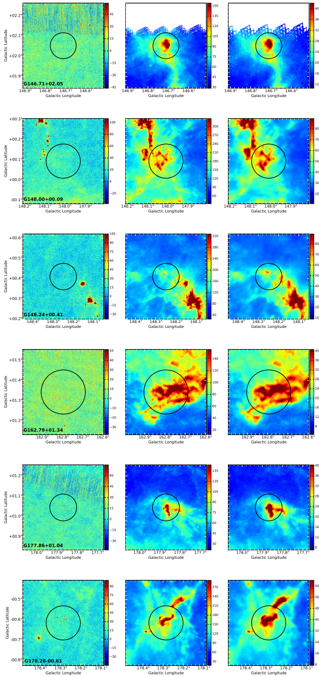
Fig. A.3. Herschel 70, 250, and 500 \mu\text{m} images of the selected Planck cold clumps given in units of MJy/sr with a resolution of 5'', 18'', and 36''. Black circles are centered at the positions of the Planck clumps and circle sizes correspond to the derived major axis of the clumps.
