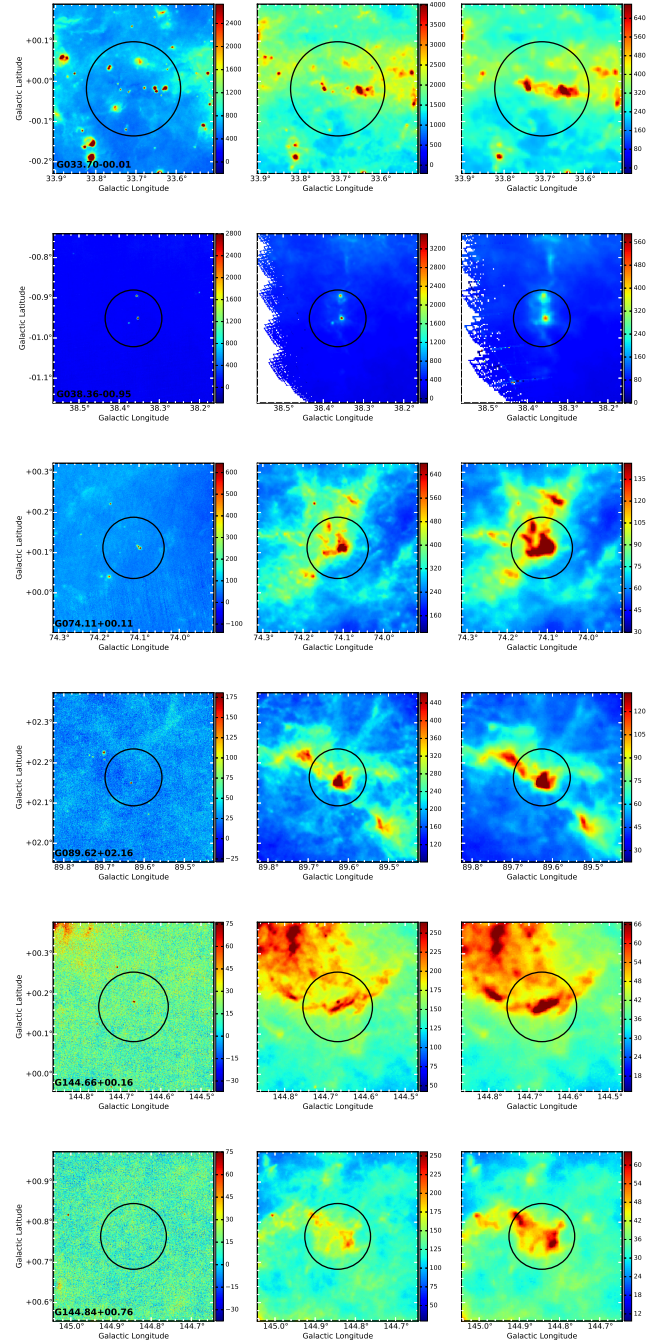
Fig. A.2. Herschel 70, 250, and 500 \mu\text{m} images of the selected Planck cold clumps given in units of MJy/sr with a resolution of 5'', 18'', and 36''. Black circles are centered at the positions of the Planck clumps and circle sizes correspond to the derived major axis of the clumps.
