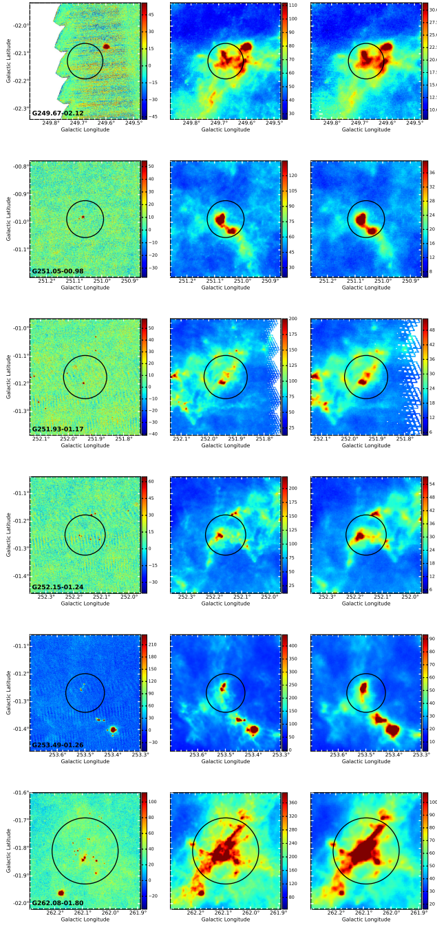
Fig. A.7. Herschel 70, 250, and 500 \mu\text{m} images of the selected Planck cold clumps given in units of MJy/sr with a resolution of 5'', 18'', and 36''. Black circles are centered at the positions of the Planck clumps and circle sizes correspond to the derived major axis of the clumps.
