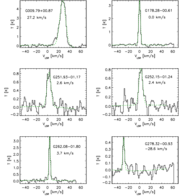
Fig. 1. Sample of CfA spectra toward the ECC clumps outside the Wu et al. (2012) survey. Green line shows the fitted Gaussian component centered at the velocity shown in the top left panel.
