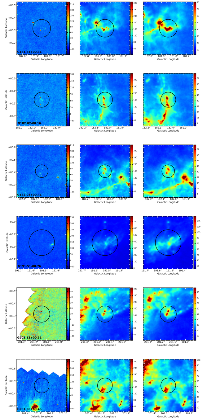
Fig. A.4. Herschel 70, 250, and 500 \mu\text{m} images of the selected Planck cold clumps given in units of MJy/sr with a resolution of 5'', 18'', and 36''. Black circles are centered at the positions of the Planck clumps and circle sizes correspond to the derived major axis of the clumps.
