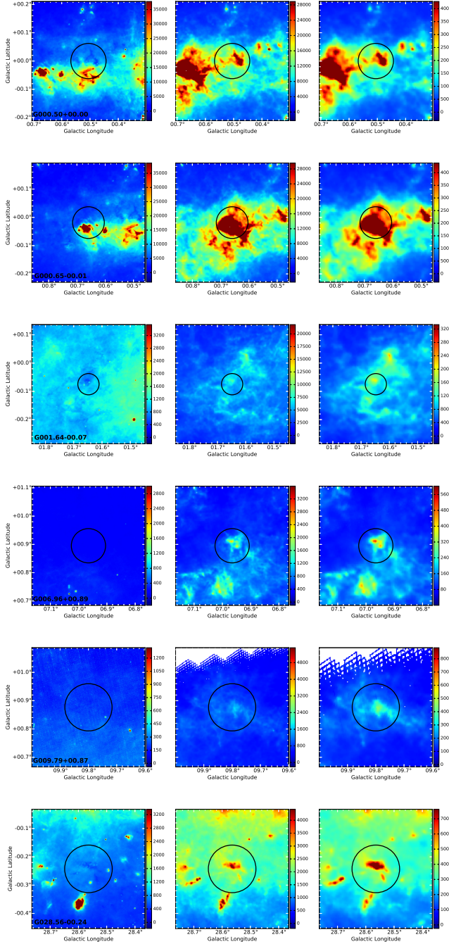
Fig. A.1. Herschel 70, 250, and 500 \mu\text{m} images of the selected Planck cold clumps given in units of MJy/sr with a resolution of 5'', 18'', and 36''. Black circles are centered at the positions of the Planck clumps and circle sizes correspond to the derived major axis of the clumps.
