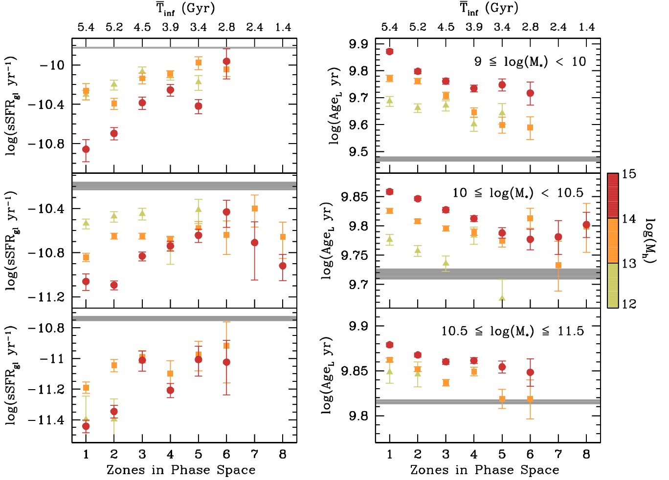
Figure 11. The observed distribution of average global sSFR and average age of our sample satellites as a function of zone and \bar{T}_{\text{inf}} in projected phase space in the left- and right-hand columns, respectively. The error bars represent the error on the mean. Satellites are split into three bins of stellar mass (from 10^9 to 10^{11.5} M_{\odot} h^{-2} ) and three bins of halo mass: 12 \leq \log[M_h (M_{\odot} h^{-1})] < 13 (yellow triangles), 13 \leq \log[M_h (M_{\odot} h^{-1})] < 14 (orange squares), and 14 \leq \log[M_h (M_{\odot} h^{-1})] \leq 15 (red circles). Each grey shaded area represents the range in weighted mean sSFR gl and Age L spanned by field galaxies.
