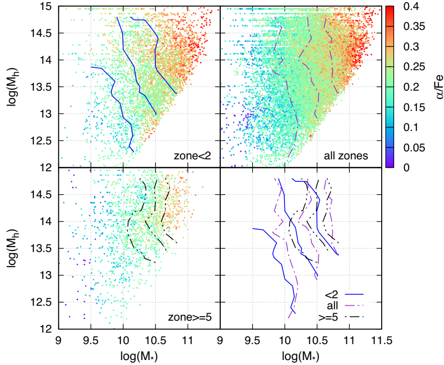
Figure 10. As in Fig. 6 but for [\alpha/\text{Fe}] element ratio instead of sSFR. Contours are shown at [\alpha/\text{Fe}] = 0.2, 0.24 , and 0.275 (from left to right). Galaxies in zone \leq 2 have \bar{T}_{\text{inf}} \geq 5 Gyr, while those in zone \geq 5 have \bar{T}_{\text{inf}} \leq 3.4 Gyr.
