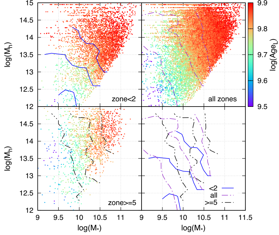
Figure 8. As in Fig. 6 but for luminosity-weighted age instead of sSFR. Contours are shown at \log(\text{Age}_L) = 9.7, 9.8, \text{ and } 9.85 (from left to right). Galaxies in zone \leq 2 have \bar{T}_{\text{inf}} \geq 5 Gyr, while those in zone \geq 5 have \bar{T}_{\text{inf}} \leq 3.4 Gyr.
