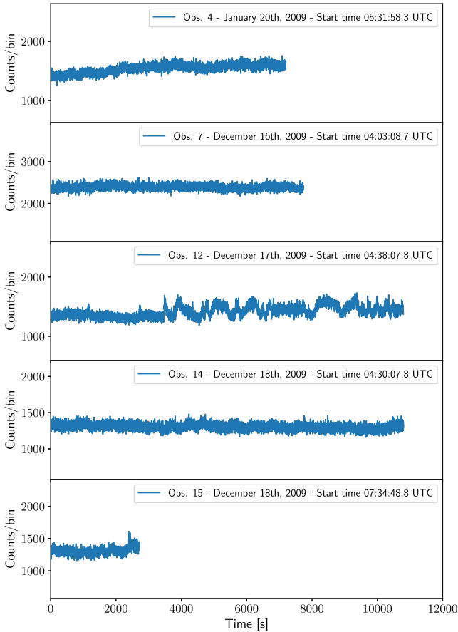
Figure 1. Light curves with time bin of 1 s of the five observations with the most significant signal (see Table 1 and the text for details).
