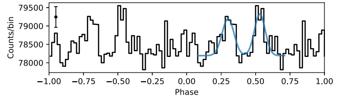
Figure 2. One of the 45 min segments of Obs. 12 folded with the period P_{\text{init}} = 0.089\,366\,94 s. The blue line shows two Gaussian functions used to fit the main optical peaks. The average 1\sigma error bar is shown on the top left.
