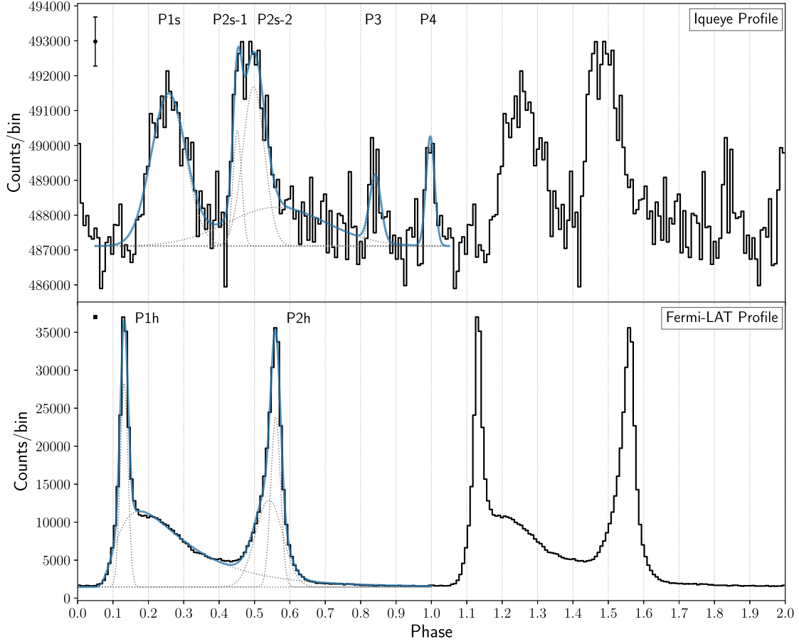
Figure 4. Two periods of the Vela pulsar pulse profile from the Iqueye optical observations taken in 2009 ( top panel ) and the Fermi -LAT gamma-ray observations taken during 3 yr of its operation (MJD 54682.66–55793.85, bottom panel ). The blue line in each plot shows the best-fitting analytical function which reproduces the profile. Individual components of these functions are also shown with grey dashed lines. Phase 0 corresponds to the radio peak. The average 1\sigma error bar is shown on the top left.
