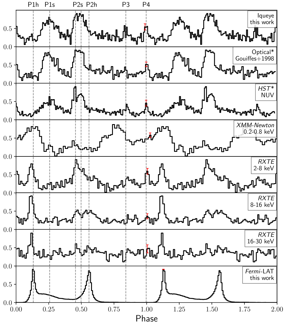
Figure 5. Normalized pulse profiles of the Vela pulsar in different energy bands. Optical, near UV, and X-ray profiles are adopted from Gouiffes (1998), Romani et al. (2005), and Kuiper & Hermesen (2015) and Harding et al. (2002), respectively. Pulse profiles from Gouiffes (1998) and Romani et al. (2005) (marked with asterisks) are shifted so as to align them with the Iqueye profile (see the text for details). Phase 0 corresponds to the radio peak. The vertical dotted lines mark the positions of different peaks. The average 1\sigma error bar for each profile is shown in red.
