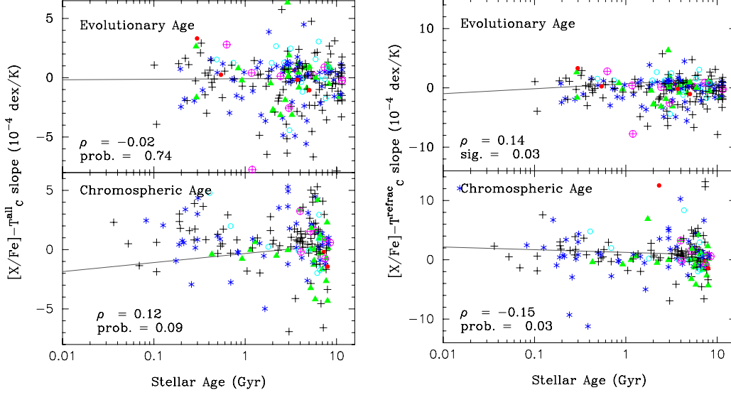
Fig. 11. T_C^{\text{all}} -slope (left) and T_C^{\text{refrac}} -slope (right) as a function of the \log R'_{HK} -derived ages (bottom panels) and isochrone ages (top panels). A linear fit to the data is shown by the grey continuous line. Results from the Spearman's correlation test are also shown in the plot. Colours and symbols are as in Fig. 4.
