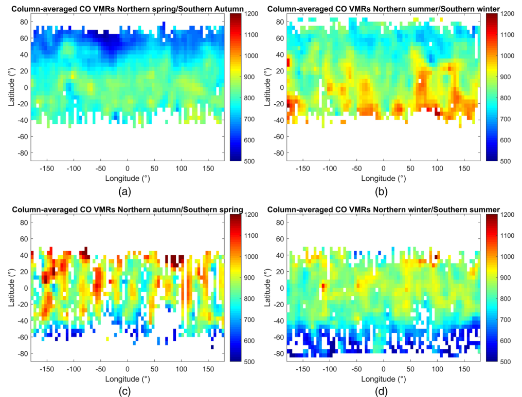
Figure 6. Distribution of CO column-averaged VMRs (ppm) retrieved from PFS spectra for each season (Northern spring L_S = [0^\circ\text{--}90^\circ] , Northern summer L_S = [90^\circ\text{--}180^\circ] , Northern autumn L_S = [180^\circ\text{--}270^\circ] , Northern winter L_S = [270^\circ\text{--}360^\circ] ). The longitudes are East. Note that the distribution is smoothed to better reveal the main patterns of seasonality. The smoothing used is the same as in Figure 3. PFS, Planetary Fourier Spectrometer; CO, carbon monoxide; VMRs, volume mixing ratios.
