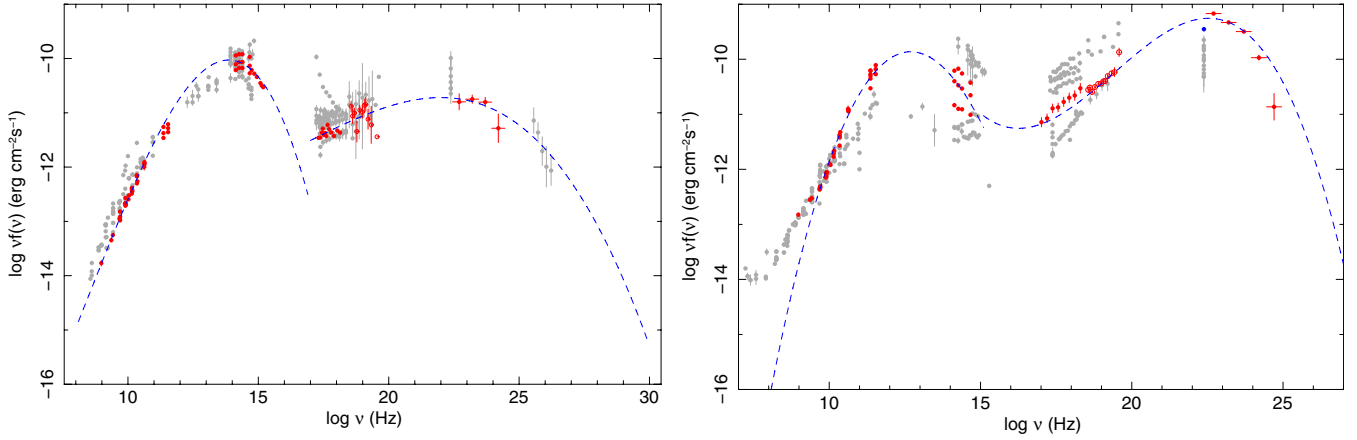
Figure 23. SED of 0FGL J2202.4+4217 = BL Lacertae (left) and of 0FGL J2254.0+1609 = 3C454.3 (right). (A color version of this figure is available in the online journal.)
