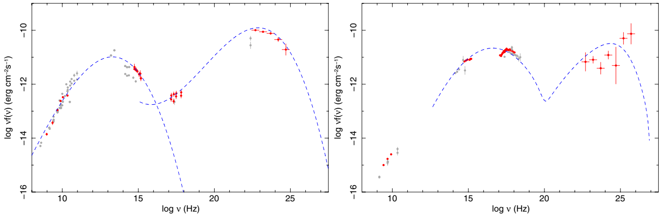
Figure 7. SED of 0FGL J0457.1–2325 = PKS0454-234 (left) and of 0FGL J0507.9+6739 = 1ES 0502+675 (right). (A color version of this figure is available in the online journal.)
