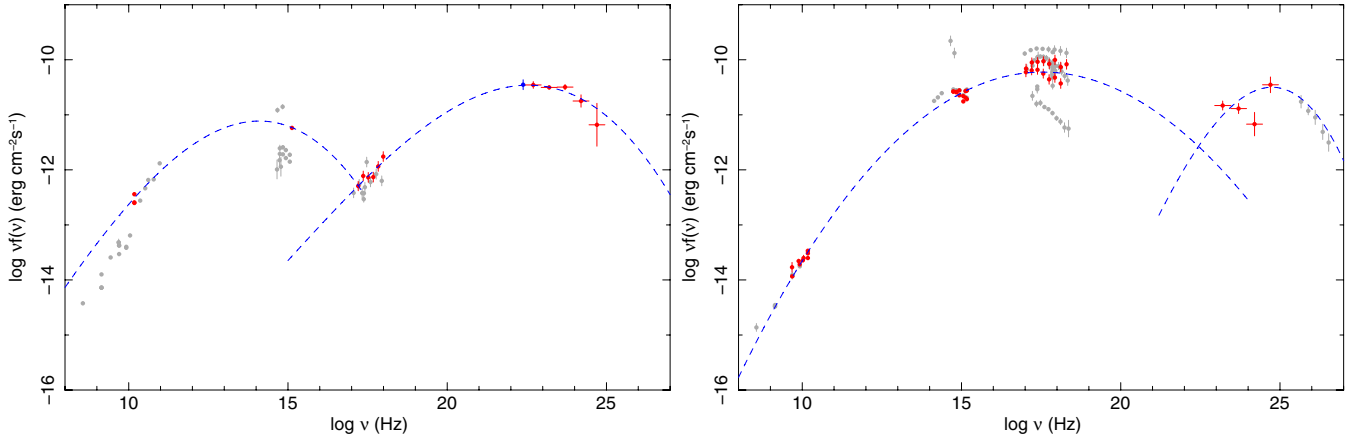
Figure 21. SED of 0FGL J1849.4+6706 = 4C66.20 (left) and of 0FGL J2000.2+6506 = 1ES1959+650 (right). (A color version of this figure is available in the online journal.)
