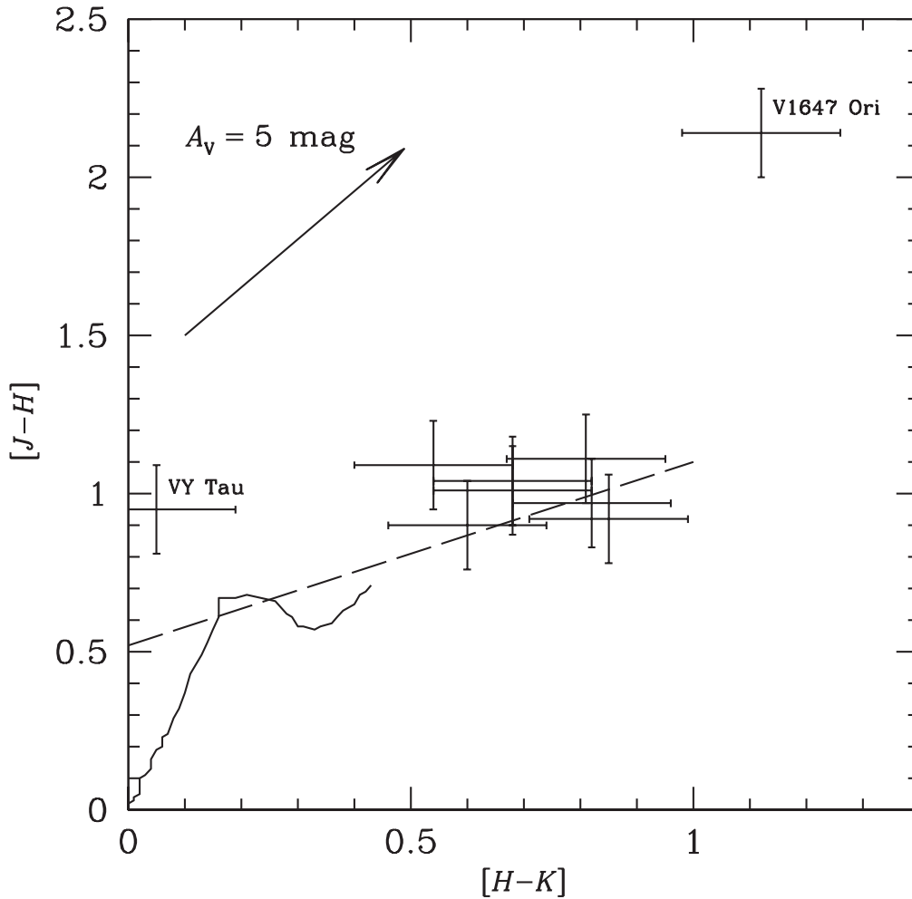
Figure 10. [J-H] vs. [H-K] color-color diagram. The arrow shows the extinction vector for A_V = 5 mag, according to the reddening law by Cardelli et al. (1989). The dashed line marks the locus of the unreddened T Tauri stars (Meyer et al. 1997), while the continuous line represents main sequence stars (Luhman et al. 2010). Data points of the objects discussed in the text are labeled.
