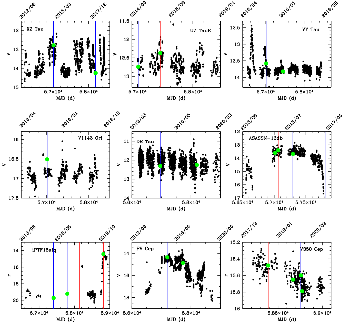
Figure 1. Optical (V- or r -band) light curves retrieved from data of public surveys (ZTF, ASASSN, and AAVSO). The x-axis represents the Modified Julian Date (MJD), while some calendar dates are given on top as reference. A blue (red) vertical line indicates the date of a MODS (LUCI) observation. The black line corresponds to quasi-simultaneous MODS+LUCI observation of DR Tau. Photometry taken closest in time to the spectroscopic observation is marked with a green dot.
