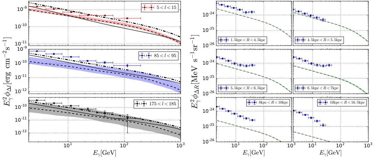
Figure 4. Case (1): fully ionized medium with n_i = 0.45 \text{ cm}^{-3} . Left panel: spectral energy distribution of the total gamma-ray emission E_\gamma^2 \times \phi_\Delta in three different angular sectors, 5^\circ \leq l \leq 15^\circ (top), 85^\circ \leq l \leq 95^\circ (centre) and 175^\circ \leq l \leq 185^\circ (bottom). The black dashed line corresponds to the mean value, while the band corresponds to a confidence level of 68%. The solid line corresponds to the mean diffuse gamma-ray emission, while the dash-dot-dot line corresponds to the sum of the average gamma-ray emission produced by self-confined CRs with the mean diffuse gamma-ray emission (sum of the dashed and the solid lines). The data points are from Yang et al. (2016). Right panel: the spectral energy distribution of the total gamma-ray emission per H atom, E_\gamma^2 \times \phi_{\Delta R} , in six different ring sectors (see labels). The black dashed line corresponds to the mean value, while the band corresponds to a confidence level of 68%. The data points are from Acero et al. (2016).
