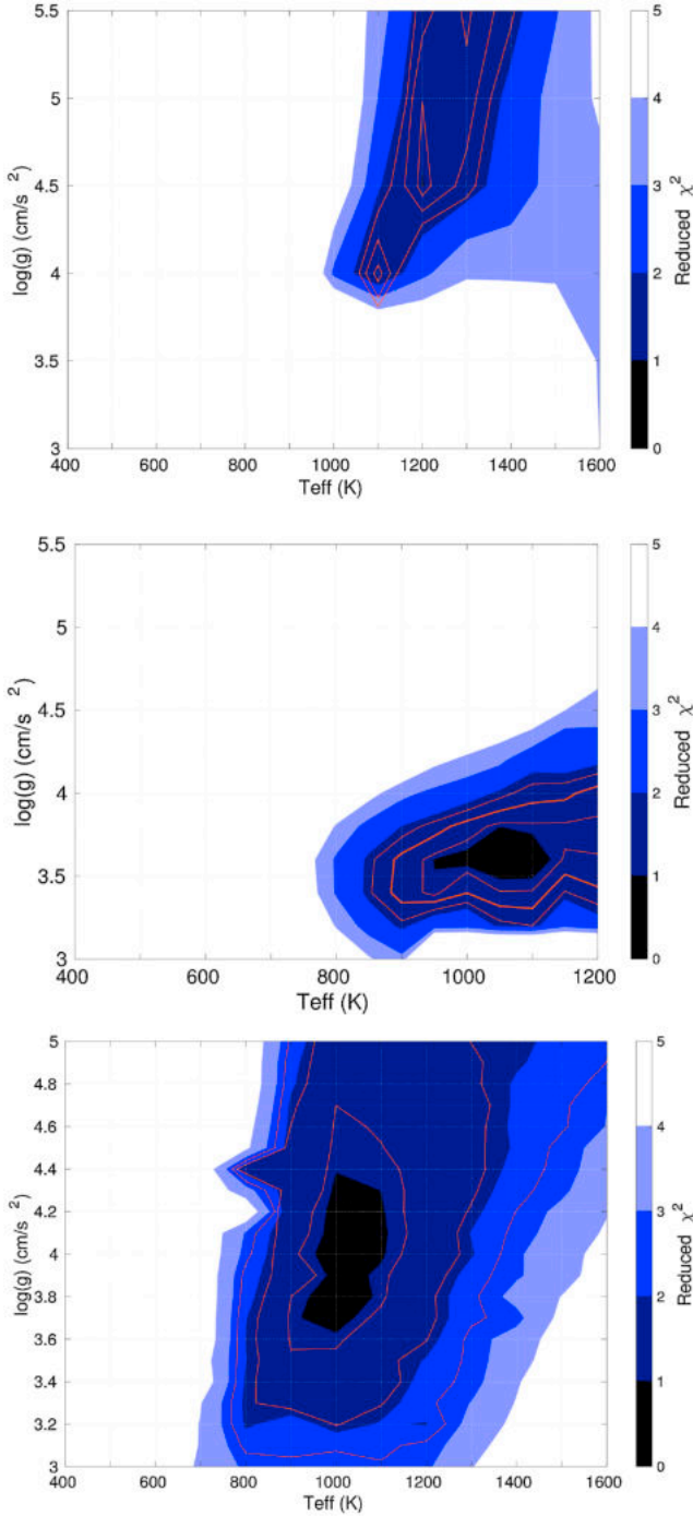
Fig. 10. Reduced \chi^2 contour map of the BT-Settl (top), Exo-REM (middle), and Exo-REM modified cloud (bottom) models. All the plots shown here are for solar metallicities. The red contours are for 1, 3, and 5\sigma .
