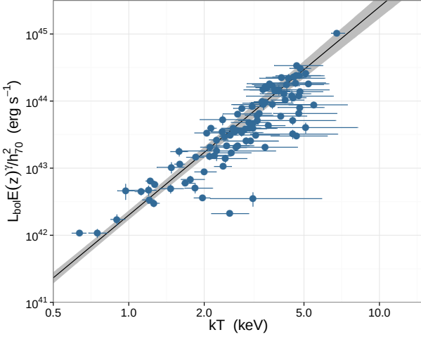
Fig. 8: L_{bol} - T relation with best-fitting model. Our best-fitting model is shown as the solid black line with the grey shading indicating the 1\sigma uncertainty. The best-fitting model is transformed from the soft band to bolometric via the steps described in Sect. 4.7.
