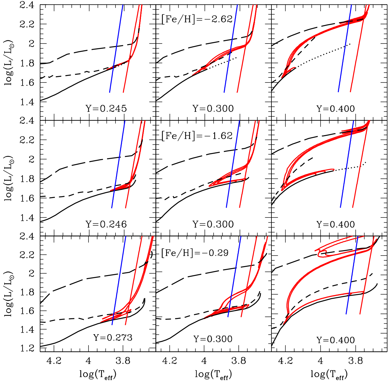
Figure 1. Hertzsprung–Russell diagrams of low-mass helium burning stellar structures. Top—from left to right evolutionary prescriptions for a metal-poor iron abundance (see labeled value) and three different helium contents. The solid lines display the zero-age horizontal branch (ZAHB), while the dotted lines show the extension to younger progenitors until the crossing of the RRL IS. The dashed and the long-dashed lines display the 90% and the 100% central helium exhaustion. The red solid lines display three HB evolutionary models covering the mass range typical of RRLs located close to the blue edge, to the middle of the IS, and to the red edge of the IS. The blue and the red, almost vertical, lines show the blue and the red edge of the predicted RRL IS. Middle—same as the top, but for a metal-intermediate chemical composition. Bottom—same as the top, but for a more metal-rich chemical composition.
