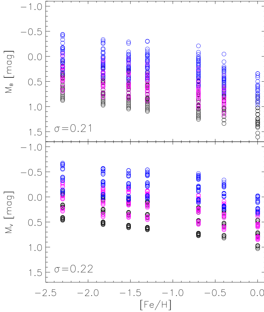
Figure 3. Top: predicted (fundamentals plus first overtones) B -band mean magnitude metallicity ( M_B – [\text{Fe}/\text{H}] ) relation. Symbols are the same as in Figure 2. The standard deviation is labeled in the bottom left corner. Bottom: same as the top, but for the M_V – [\text{Fe}/\text{H}] relation.
