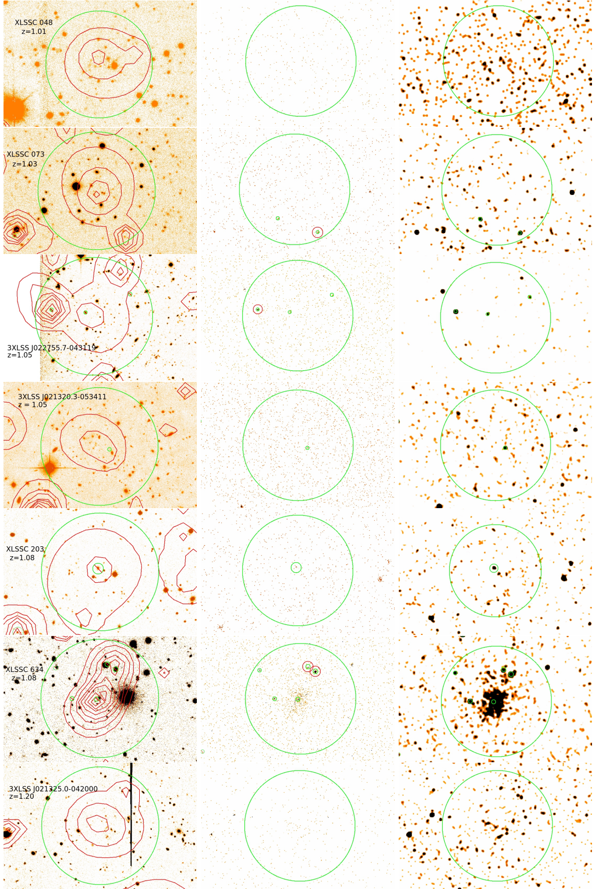
Fig. 2. Same as Fig. 1 but for all C2 clusters. All optical images are i -band images from the CFHTLS except for XLSSC 203 which is r -band and XLSSC 073 which is g -band.
