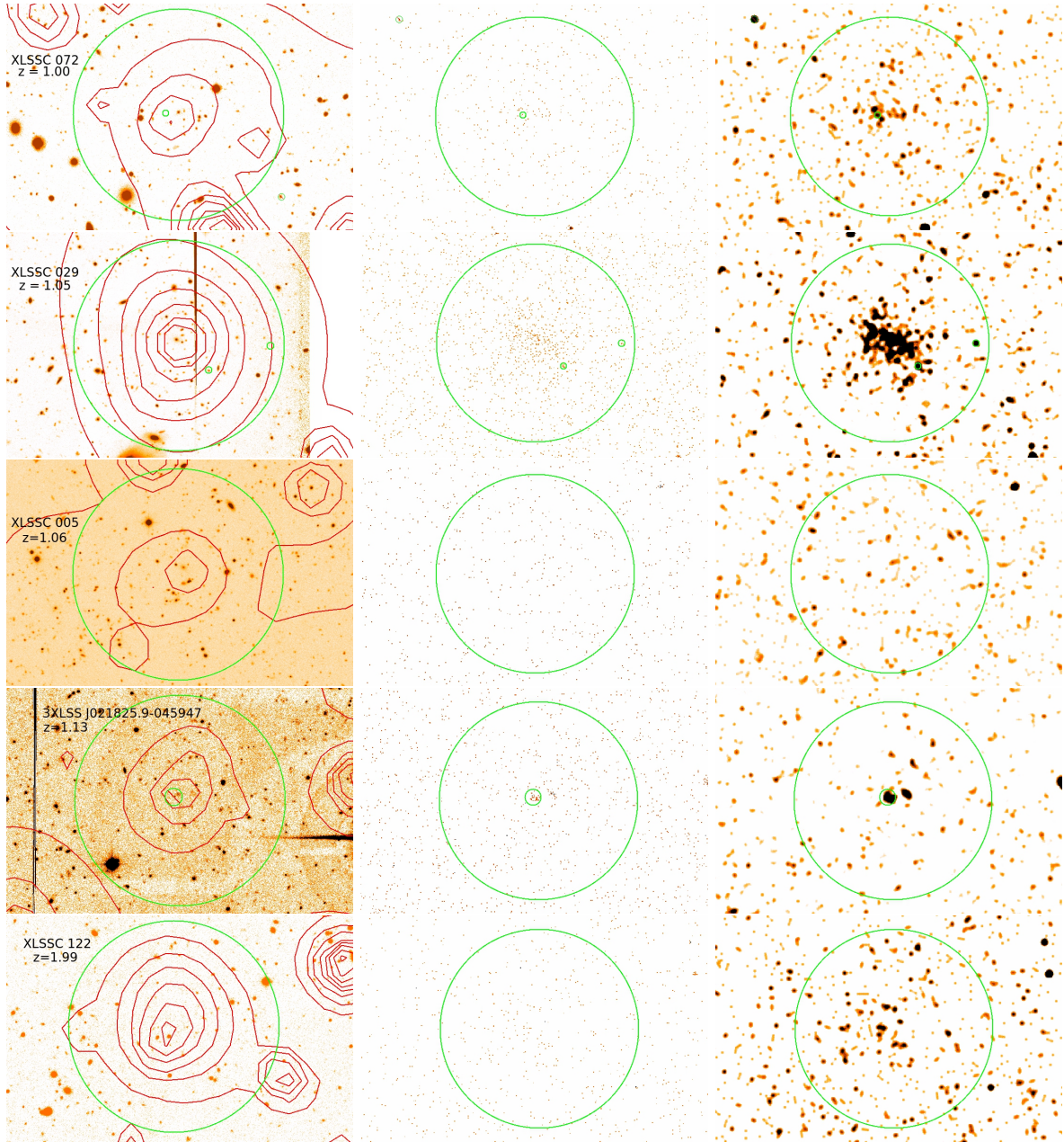
Fig. 1. A comparison of the optical image with the XMM-Newton contours from the 0.5–2 keV band (red) superimposed ( left panel ) and the raw and smoothed (using a Gaussian with \sigma \sim 2.5'' ) Chandra ( centre and right panels , respectively) images for all C1 clusters. All optical images are i -band images from the CFHTLS except for 3XLSS J021825.9-045947 which is r -band. Chandra images are in the 0.3–8.0 keV band. The green circle is the same in all images and is of radius 60'' and centred on the cluster centre. Point sources within 60'' of the cluster centre are marked by the smaller green circles in all images. In the raw Chandra images, if a Chandra point source was detected in XXL, then it is circled in red.
