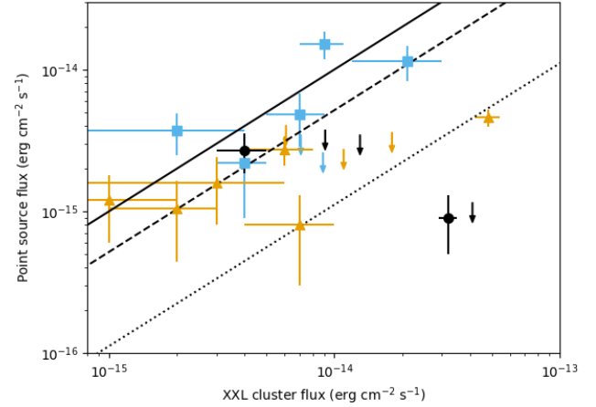
Fig. 4. Total Chandra flux for point sources within 60'' of the cluster centre versus the XMM cluster flux. C1 clusters are black circles, C2s are yellow triangles and C3s are blue squares. Arrows indicate clusters that only have a 1\sigma upper limit for their point source flux (Col. 6 in Table 2) – the tip of the arrow denotes the upper limit. The solid straight line is a line of equality showing locus of 100% AGN contamination and the dashed and dotted lines are lines of equality showing the locus of 50% and 10% AGN contamination, respectively. 1\sigma errors are shown.
