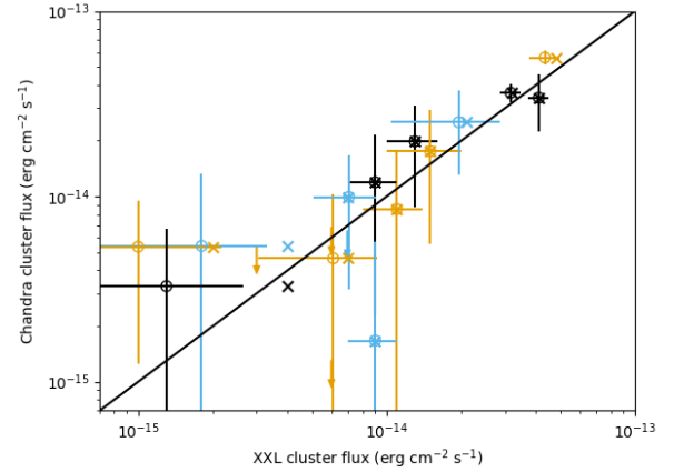
Fig. 6. Chandra cluster flux versus the XXL cluster flux, F_{60} . C1 clusters are black circles/crosses/arrows, C2s are yellow circles/crosses/arrows, and C3s are blue circles/crosses/arrows. The crosses are F_{60} as listed in Col. 4 of Table 2 (i.e. the original flux, not excluding the point sources detected by Chandra ). The circles are the F_{60} minus the flux from any point source detected in the Chandra data that was not previously resolved by XXL data (listed in Col. 6 of Table 2). The solid line is a line of equality. The arrows indicate upper limits on the Chandra cluster flux – the tip of the arrow denotes the upper limit and are plotted against the point source corrected XXL flux. 3XLSS J022059.0-043922 and 3XLSS J022554.3-045059 are not shown on the plot as the Chandra point source flux is greater than F_{60} .
