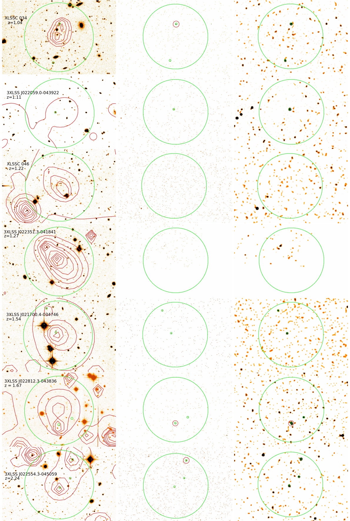
Fig. 3. Same as Fig. 1 but for all C3 clusters. All optical images are i -band images from the CFHTLS.
