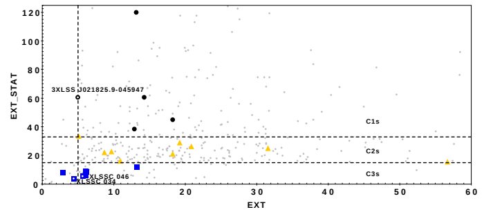
Fig. 5. EXT – EXT_STAT parameter space for the C1s, C2s, and C3s in our sample (larger black circles, yellow triangles, and blue squares, respectively). We also show a representative sample of C1, C2, and C3 XXL clusters at 0 < z < 1 for illustration (smaller grey circles). The C1/C2/C3 boundaries are explained in Sect. 2. The three larger circles/squares with the hollow centres are those with labels on the plot.
