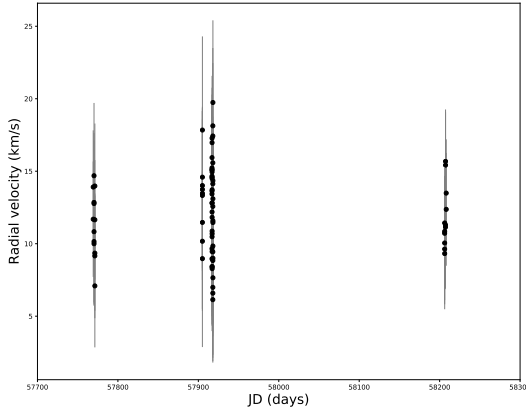
Fig. 9. Radial velocity measurements of HIP 65426 using a total of 78 HARPS spectra obtained between 2017 and 2018 at the La Silla 3.6m telescope and weak metallic lines that are less sensitive to the continuum tracing.
