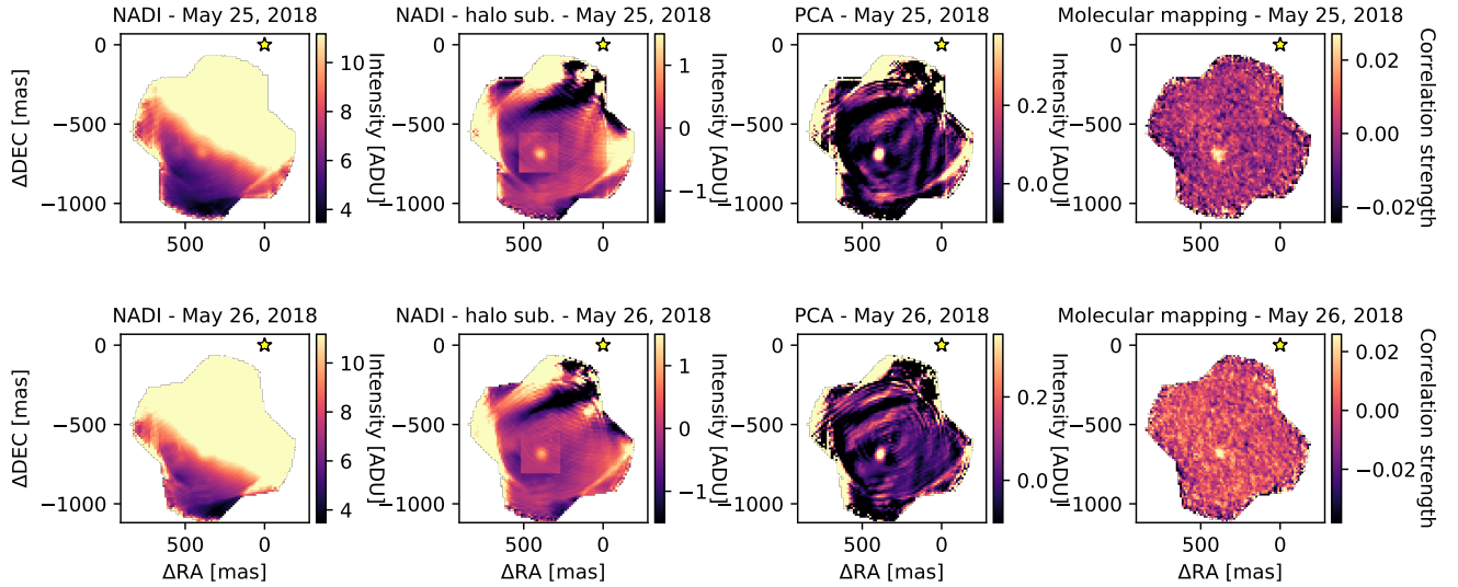
Fig. 1. Detection of HIP 65426 b with SINFONI using (from left to right) a simple derotation and stacking of the individual cubes (nADI), a removal of the halo at each wavelength using a circular profile and a local fit with a 2D polynomials, the PCA algorithm (three modes), and the molecular mapping with an Exo-REM model at T_{\text{eff}} = 1600 K, \log(g) = 4.0 dex, [M/H] = 0 dex, and C/O = 0.35 (at 20 \text{ km s}^{-1} ).
