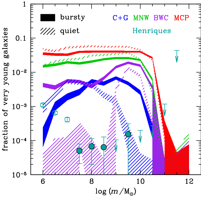
Figure 10. Effect of the galaxy merging scheme used in the analytical models on the fraction of VYGs versus stellar mass. The solid and hatched shaded regions denote the bursty and quiet merging schemes, respectively, where the weights are taken into account according to equation (23), and the errors are based upon 1000 bootstraps. The blue–green points indicate the SAM Henriques for reference (open circles) when the mass resolution is not adequate.
