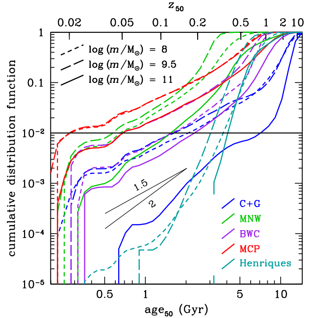
Figure 9. Cumulative distribution functions of galaxy ages for the different models (same colours as in Fig. 6) and for three different bins of stellar mass: \log(m/M_\odot) = 7.25-8.75 (short dashed), 8.75-10.25 (long dashed), and 10.25-11.75 (solid). The ages are medians (half the mass formed) for the analytical models (with the bursty galaxy merging scheme) and arithmetic means for the Henriques SAM. The short segments indicate slopes of 1.5 and 2, while the horizontal line indicates the youngest 1 per cent of galaxies.
