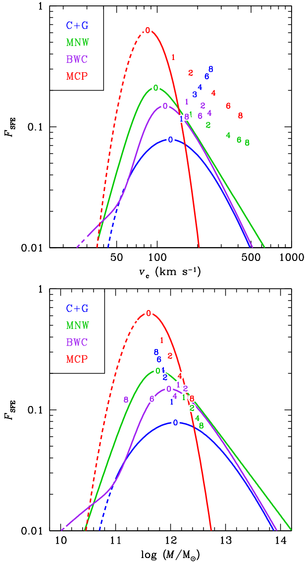
Figure 2. Star formation efficiency, F_{\text{SFE}} , of our analytical galaxy formation models versus halo circular velocity ( top ) and mass ( bottom ) at z = 0 . The blue, green, and purple curves, respectively, show F_{\text{SFE}} = \dot{m}/(f_b \dot{M}) for models C+G (Cattaneo et al. 2011 with Gnedin 2000, equations 5–7), MNW (Moster et al. 2013, equations 8 and 9), and BWC (Behroozi et al. 2013, equations 10–13). For model MCP (Mutch et al. 2013, equations 15 and 16, F_{\text{SFE}} = 0.7 \dot{m}/(f_b \dot{M}) ). The dashed portions of the curves indicate where the models are extrapolations. The numbers indicate the position of the peak SFE at the corresponding redshift.
