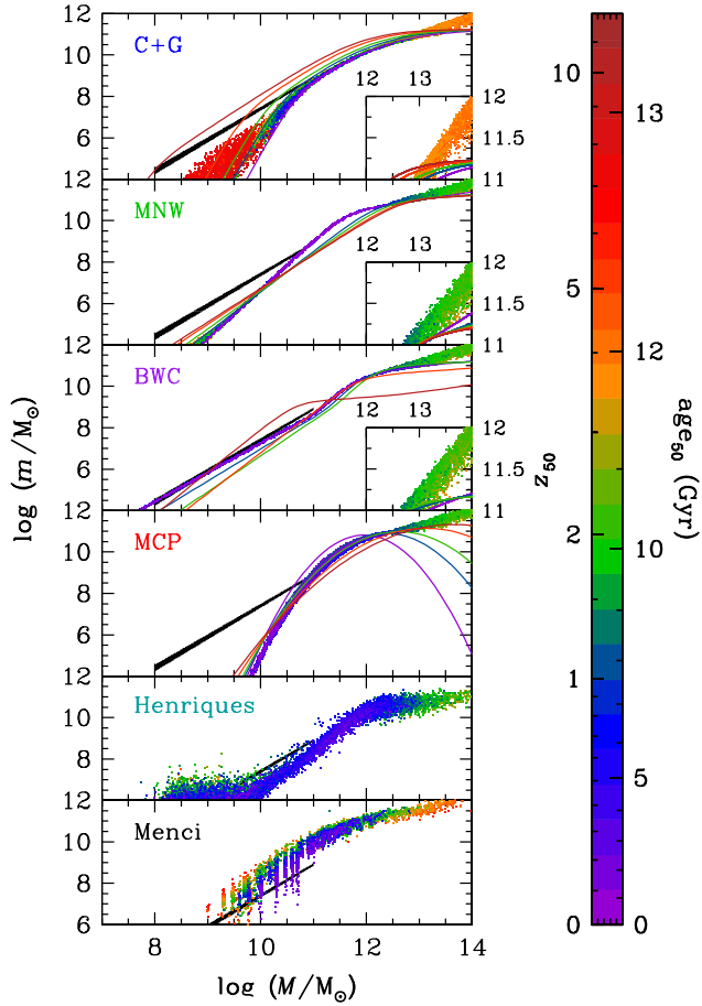
Figure 5. Stellar mass versus halo mass at z = 0 for the four analytical models (with bursty galaxy merging, top panels, see Fig. 2) and for the SAMs of Henriques and Menci (bottom two panels), restricted to centrals with galaxy stellar masses m > 10^6 M_\odot for lack of mass resolution). Each point corresponds to a galaxy extracted from the analytical or SAMs run on the halo merger trees. The points are colour coded by the median (analytical models) or mean (Henriques SAM) redshift, z_{50} , and are plotted in order of decreasing age, with violet colours for the galaxies younger than 1.3 Gyr. For clarity, only 500 galaxies are shown per 0.25 dex halo mass interval. The curves show the SMHMs directly predicted by the analytical models, with equation (1) for the C+G, MNW, and BWC models and equation (14) for the MCP model, using the SFEs illustrated in Fig. 2. These curves are given at redshifts 0, 1, 2, 5, and 10, following the same colour code as for z_{50} . The insets show 4\times vertical zooms of the high-mass end. The thick black lines show the observations of isolated dwarf irregular galaxies compiled by Read et al. (2017), with uncertainties illustrated by the line thickness.
